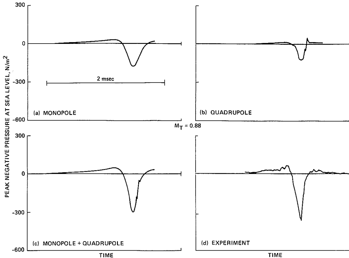
Figure 12. Theory-experiment comparison, M_{tip} = 0.88 .
