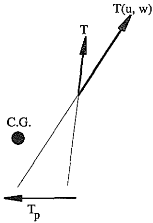
Figure 8: Rotor and Propeller Forces in Equilibrium and Disturbed Flight
