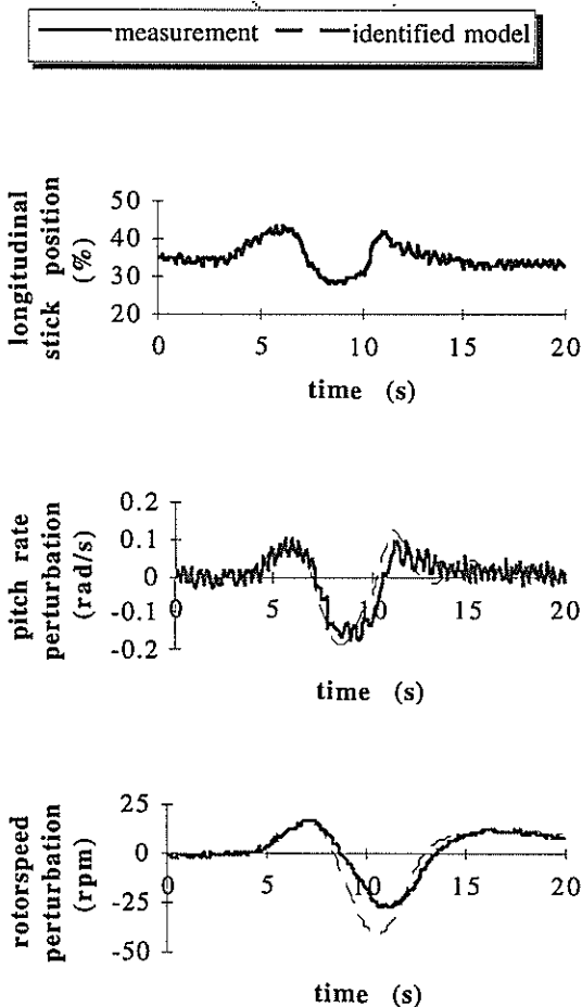
Figure 4a : Identified model verification, 70 mph, short-term response
