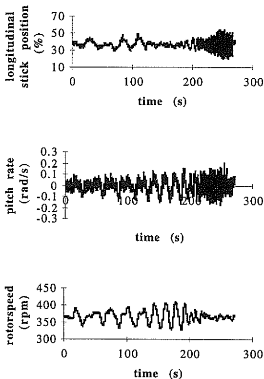
Figure 2: Response during frequency sweep test at 70 mph
