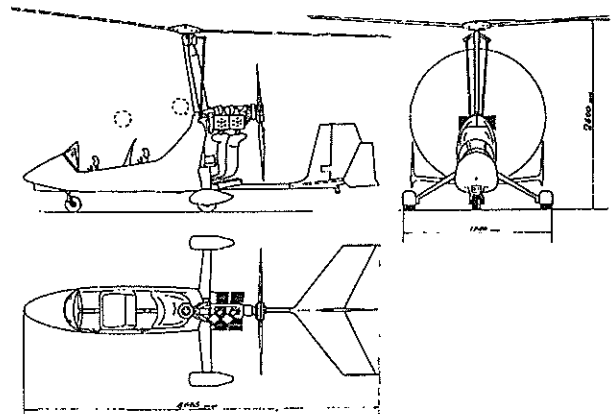
Figure 1: VPM M16 Gyroplane
