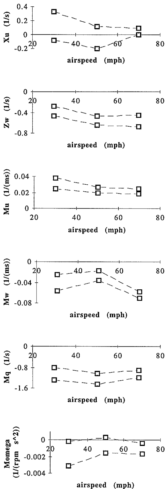
Figure 7: Key identified force and pitching moment derivatives
