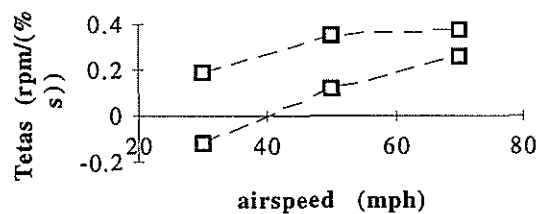
Figure 10: Rotor torque derivatives
