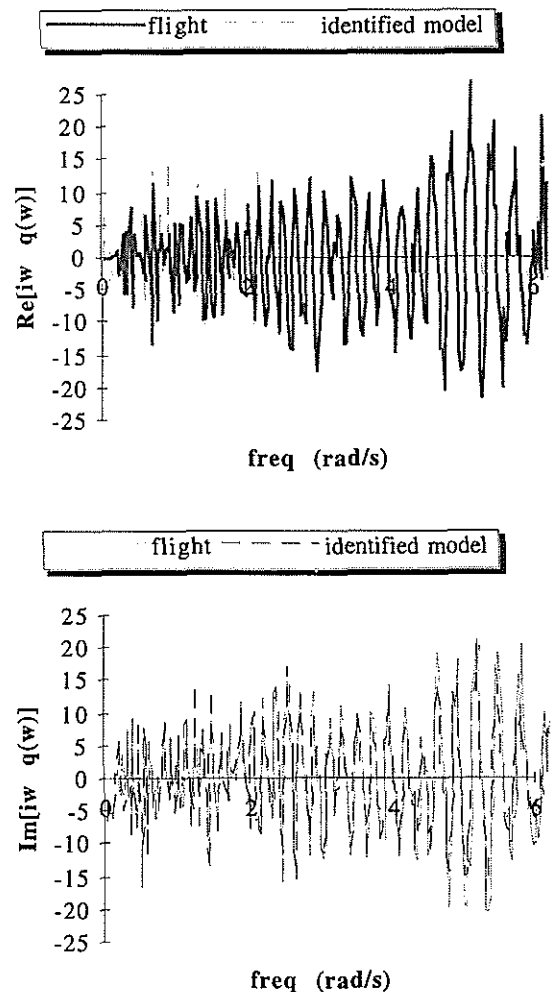
Figure 3: Fit quality - flight and identified model pitching moment equation
