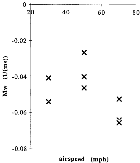
Figure 9: Multi-run consistency of result in M_w
