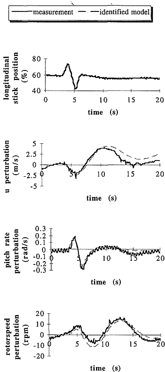
Figure 5: Identified model verification, 30 mph
