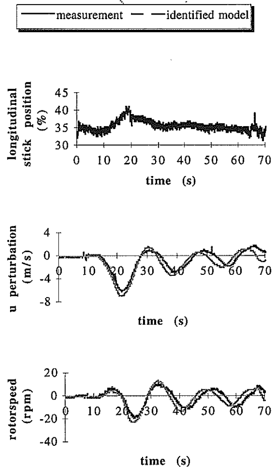
Figure 4b : Identified model verification, 70 mph, phugoid response
