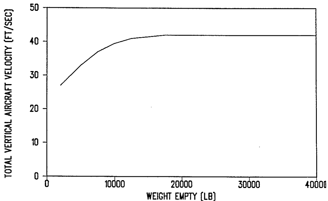
Figure 3. Suggested Vertical Crash Impact Design Condition for Total Aircraft
