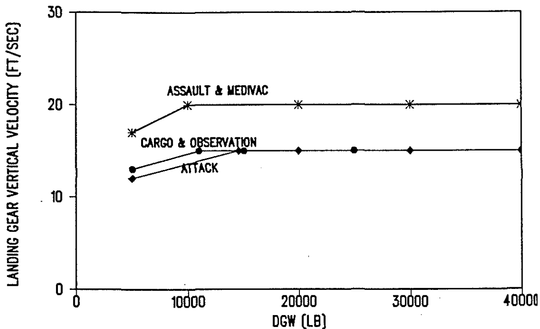
Figure 4. Suggested Vertical Crash Impact Design Condition for Landing Gear
