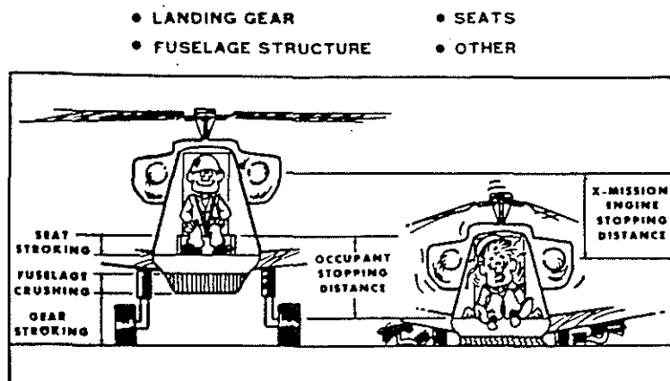
Figure 1. Energy Management System
