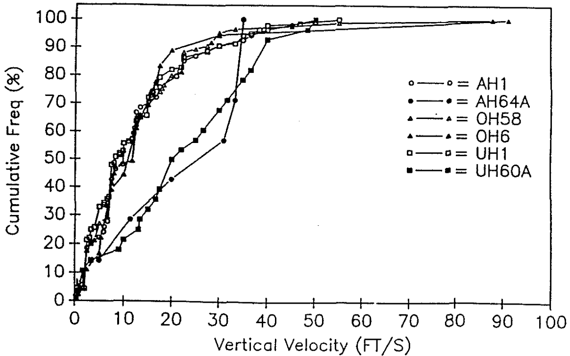
Figure 2. Army Helicopter Vertical Impact Velocity
