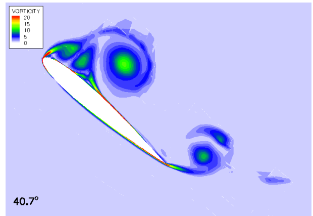
(e) leading edge vortex separates from airfoil
