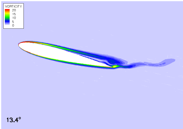
(a) separation starts at trailing edge
