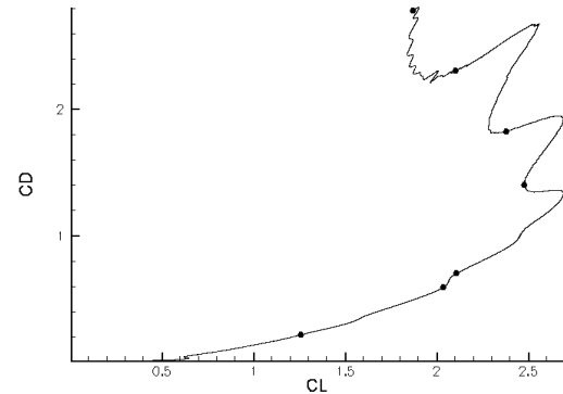
(b) CD versus CL
