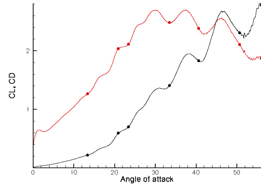
(a) CL, CD versus angle of attack
