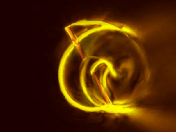
Figure 1: Simulation of the inviscid flow around the Operational Loads Survey rotor in forward flight ( M_{\text{tip}} = 0.664 , \mu = 0.164 , C_T = 0.0054 ). Vorticity magnitude (between zero and one) at an azimuth of 135^\circ . Taken from Boelens et al. [2]
