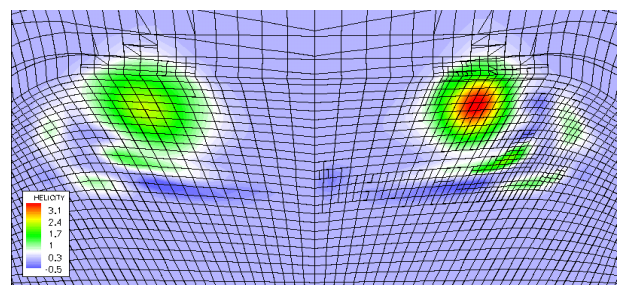
Figure 4: Vortex flow over a delta wing ( Re=40,000 , M=0.3 , \alpha = 12.5^\circ ). Comparison of vortex resolution at 10% span after trailing edge. Left unadapted results, right adapted results.
