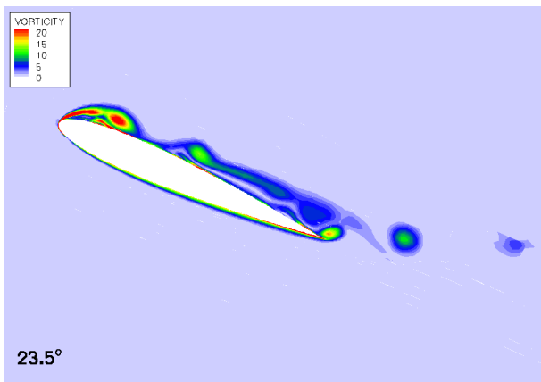
(c) boundary layer separates into several vortices
