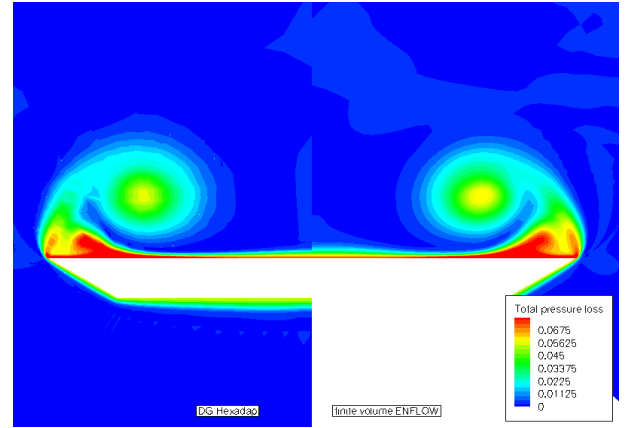
(b) total pressure loss
