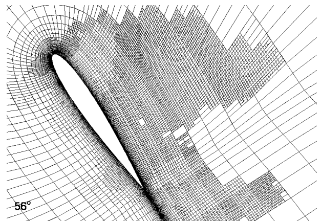
Figure 6: Laminar dynamic stall for a NACA0012 airfoil ( Re=10000 , M=0.2 ). Mesh evolution.
