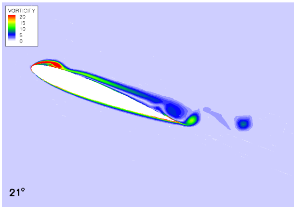
(b) leading edge separation
