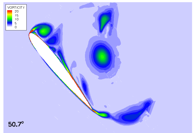
(f) rotating vortices
