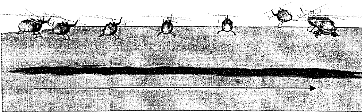
Figure 7: 3-D representation of the first part (0-15 sec) of the sidestep manoeuvre at 1 sec intervals (moving from left to right).
