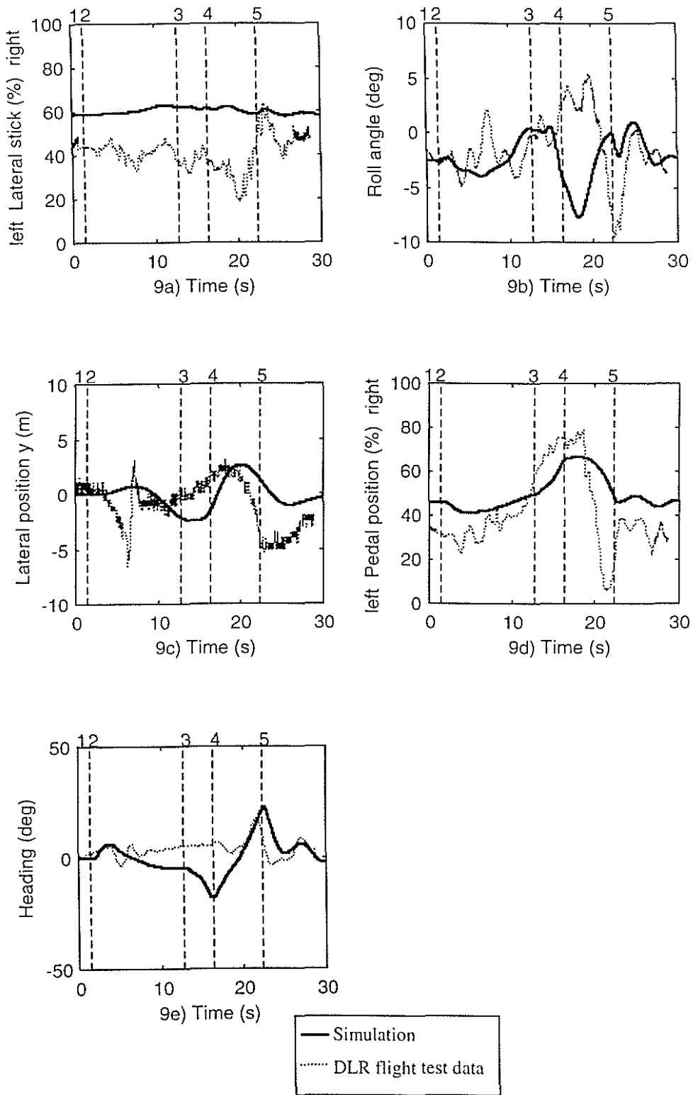
Figure 9: Off-axis responses for the accel/decel simulation.
