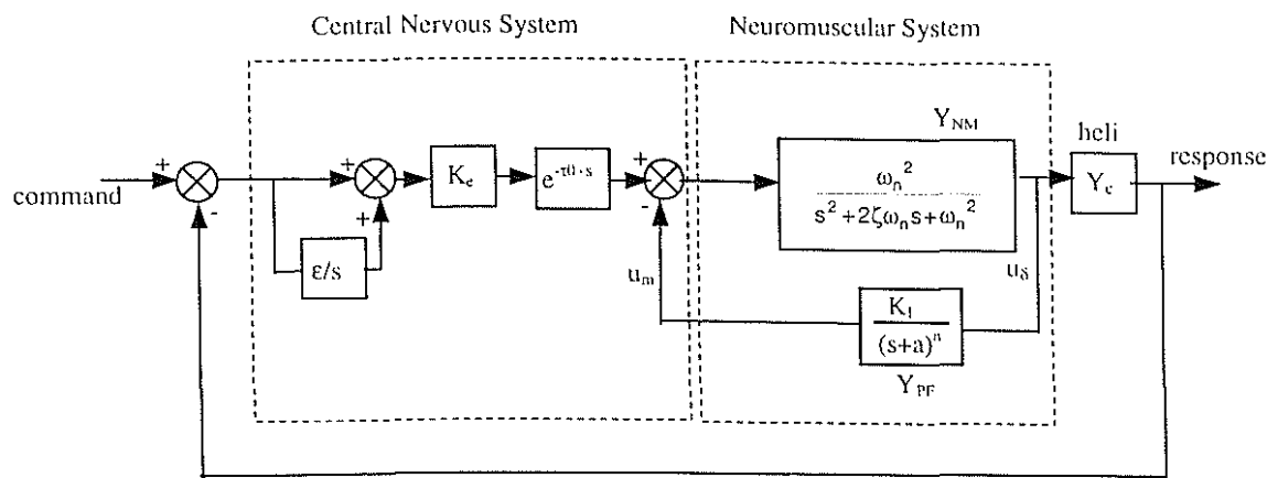
Figure 1: The Structural Pilot Model (reproduced from Ref. 1)
