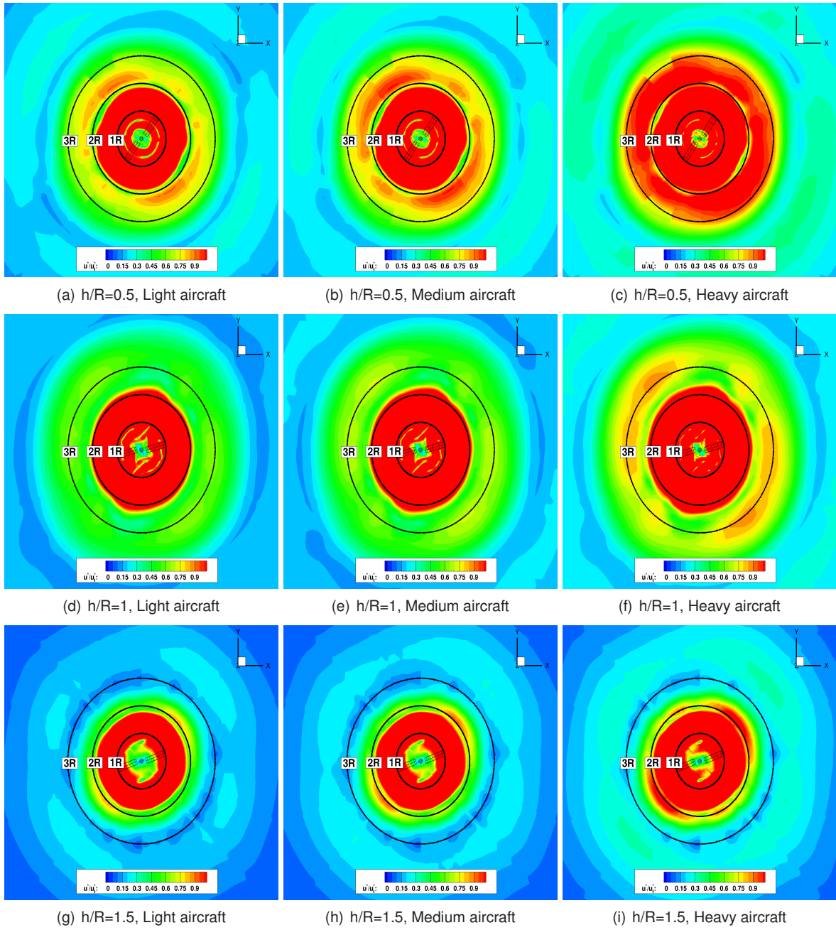
Figure 3: Uplift results for rotor at different heights above the ground and different scaling factors. All operational conditions of the small scaled rotor are listed in table 3.
