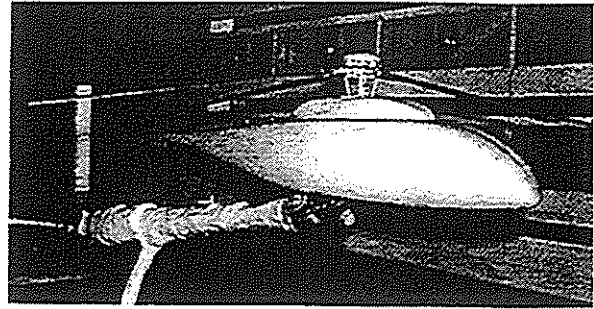
Figure 2: GRMS and Fuselage in Langley 14- by 22-Foot Subsonic Tunnel
