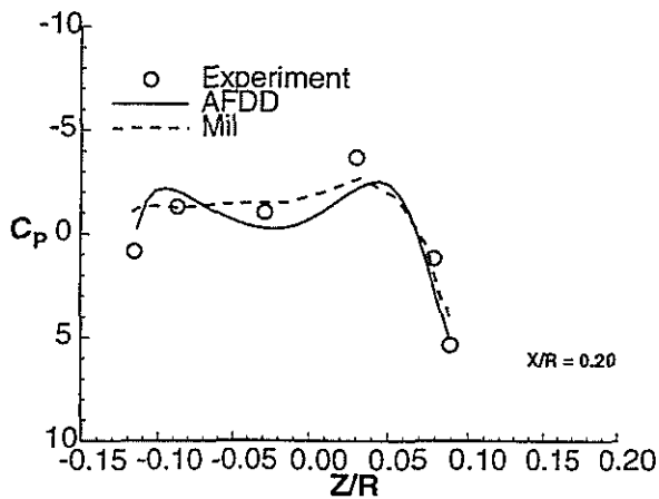
Figure 10: Pressure Comparison at X/R=0.20
