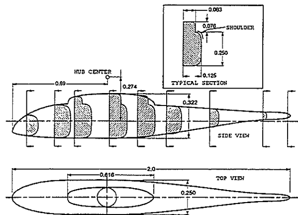
Figure 3: RO tor B ody I nteraction ( ROBIN ) Fuselage (units of rotor radius)
