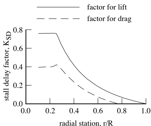
Figure 4. Stall delay factor for TRAM blade.
