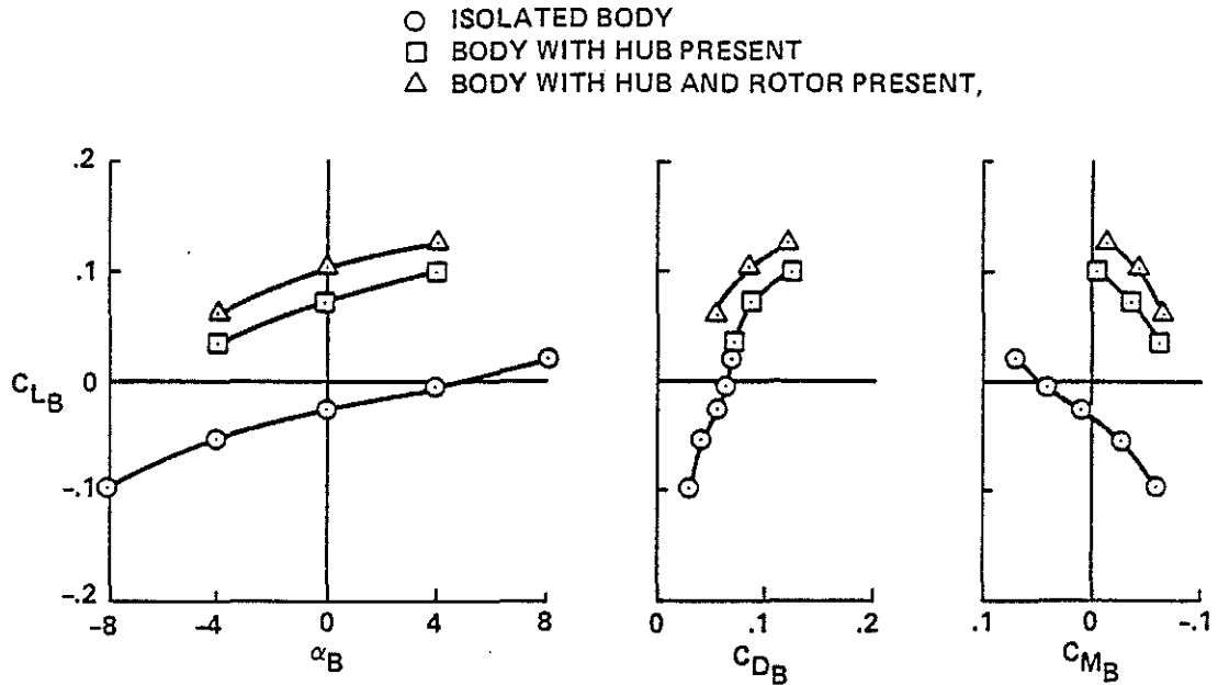
Fig. 5. Interference effect of hub and rotor on body B_2 longitudinal characteristics; baseline position, V = 61 m/sec, \mu = 0.3 , \alpha_{TPP} = 0^\circ , C_T = 0.00408 .
