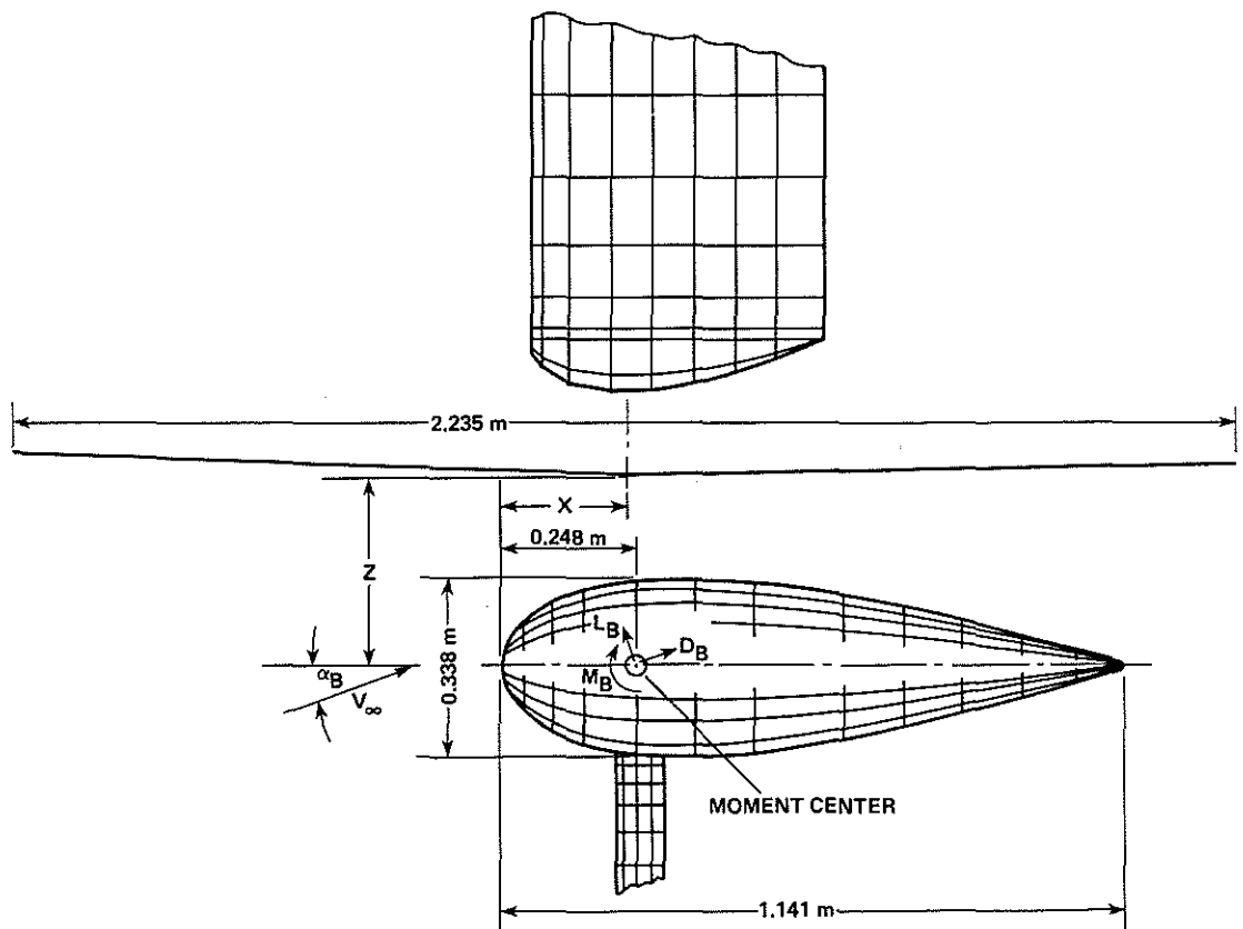
Fig. 4. Model schematic.
