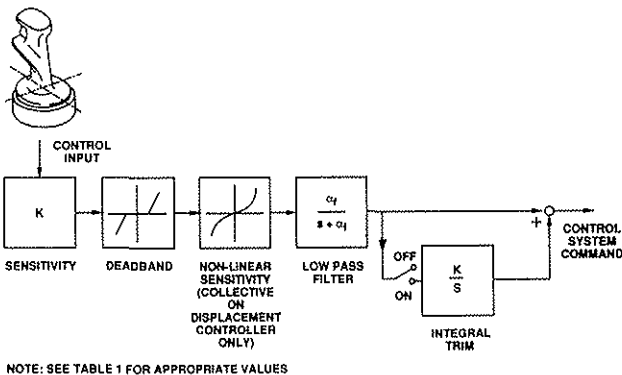
FIG. 4: CONTROL INPUT CONDITIONING
