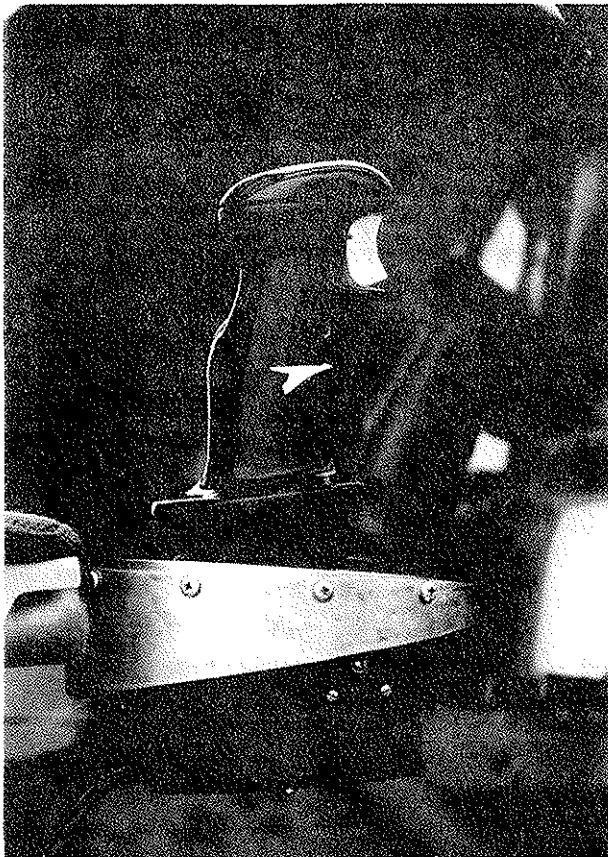
FIG. 7: FORCE SENSING SIDEARM CONTROLLER
