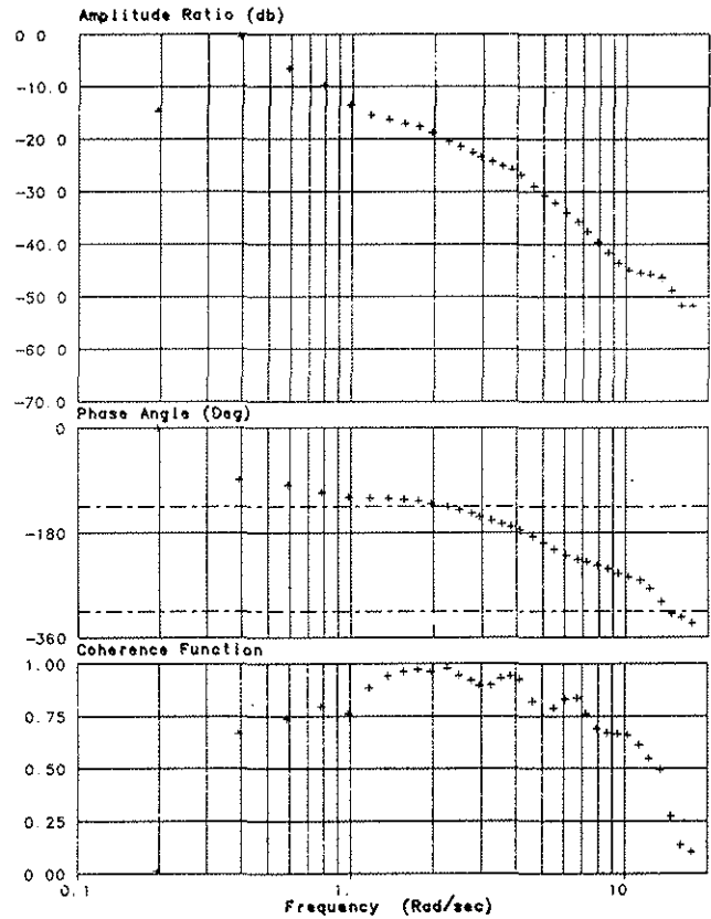
FIG. 3: ROLL AXIS BODE PLOT, \delta_\phi TO \phi (RAD) (HOVER FLIGHT CONDITION)
