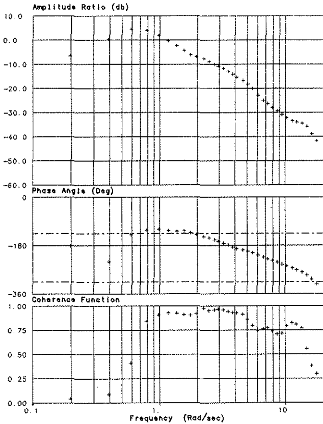
FIG. 2: PITCH AXIS BODE PLOT, \delta_\theta TO \theta (RAD) (HOVER FLIGHT CONDITION)
