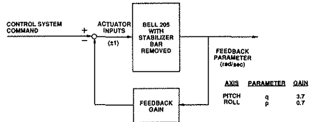
FIG. 5: PITCH AND ROLL CONTROL SYSTEM ARCHITECTURES
