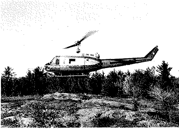
FIG. 1: THE NAE BELL 205 AIRBORNE SIMULATOR
