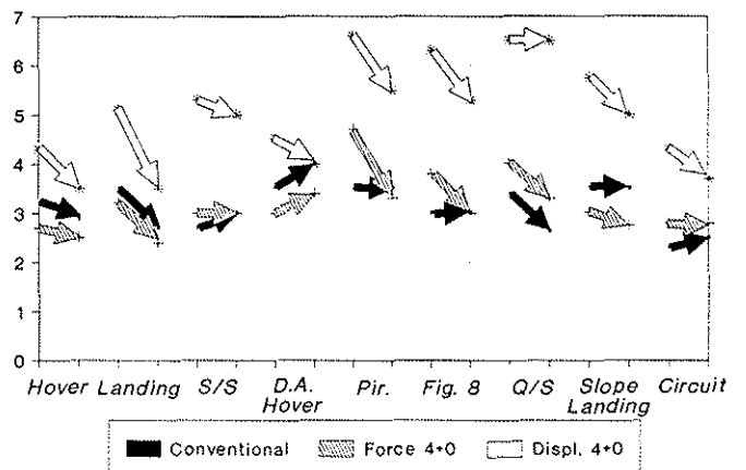
FIG. 24: LEARNING TRENDS ON INTEGRATED SIDEARM CONTROLLERS
