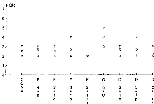
FIG. 21: OBSTACLE CLEARANCE TAKEOFF AND STEEP APPROACH RATINGS
