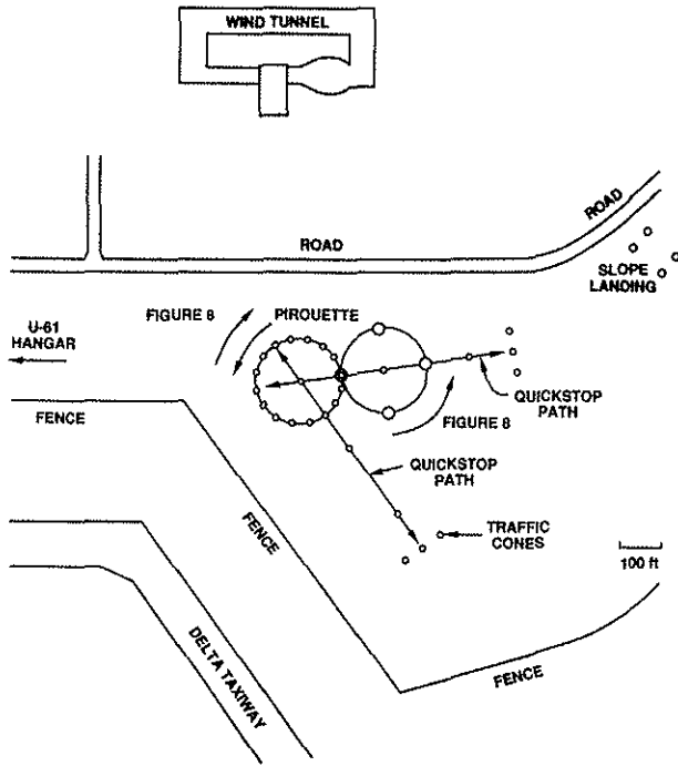
FIG. 12: EVALUATION COURSE
