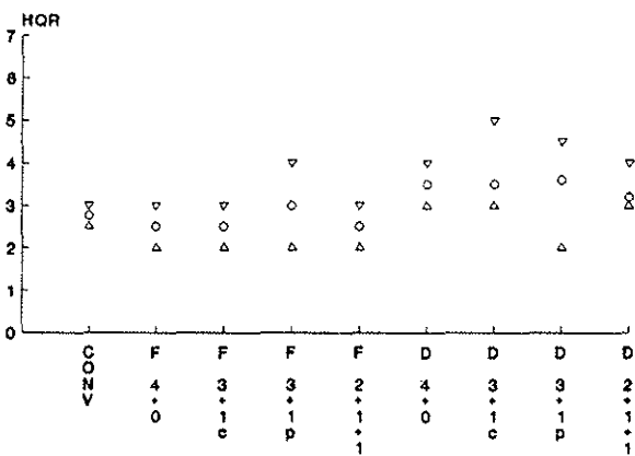
FIG. 13: HOVER RATINGS
