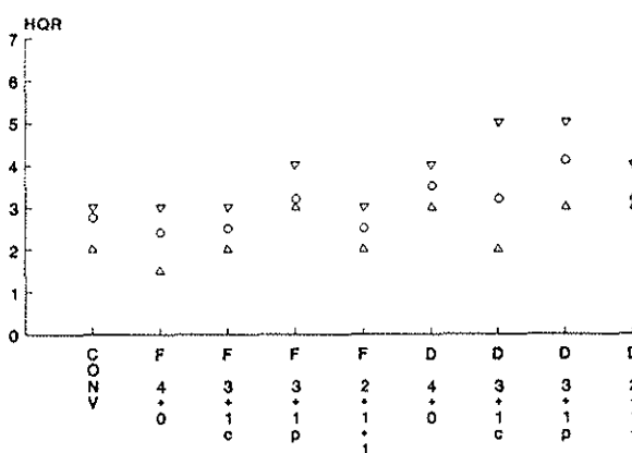
FIG. 14: LANDING RATINGS
