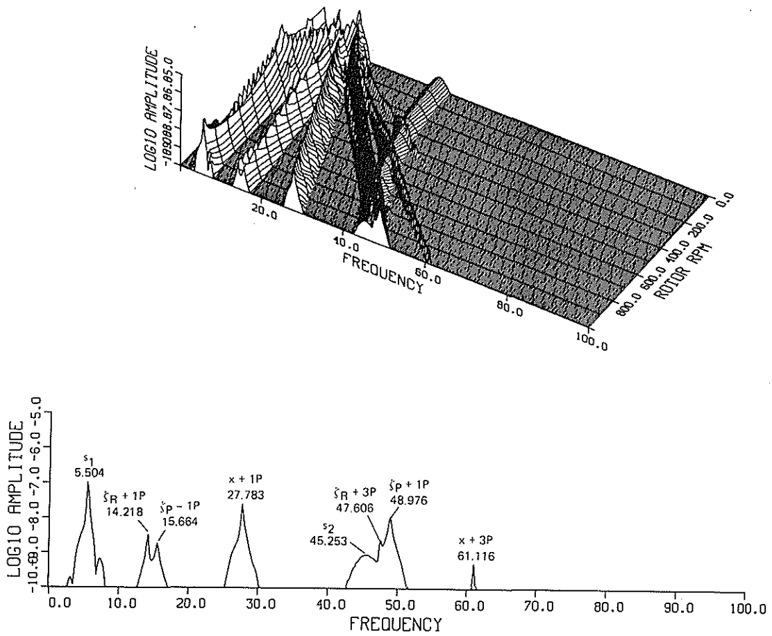
Fig. 15. Response of \zeta_o coordinate to an x initial condition; soft body, with shaft degree of freedom, 4% mismatched blades. (a) As function of rpm. (b) At 1000 rpm.
