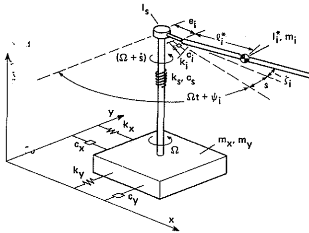
Fig. 1. System schematic.
