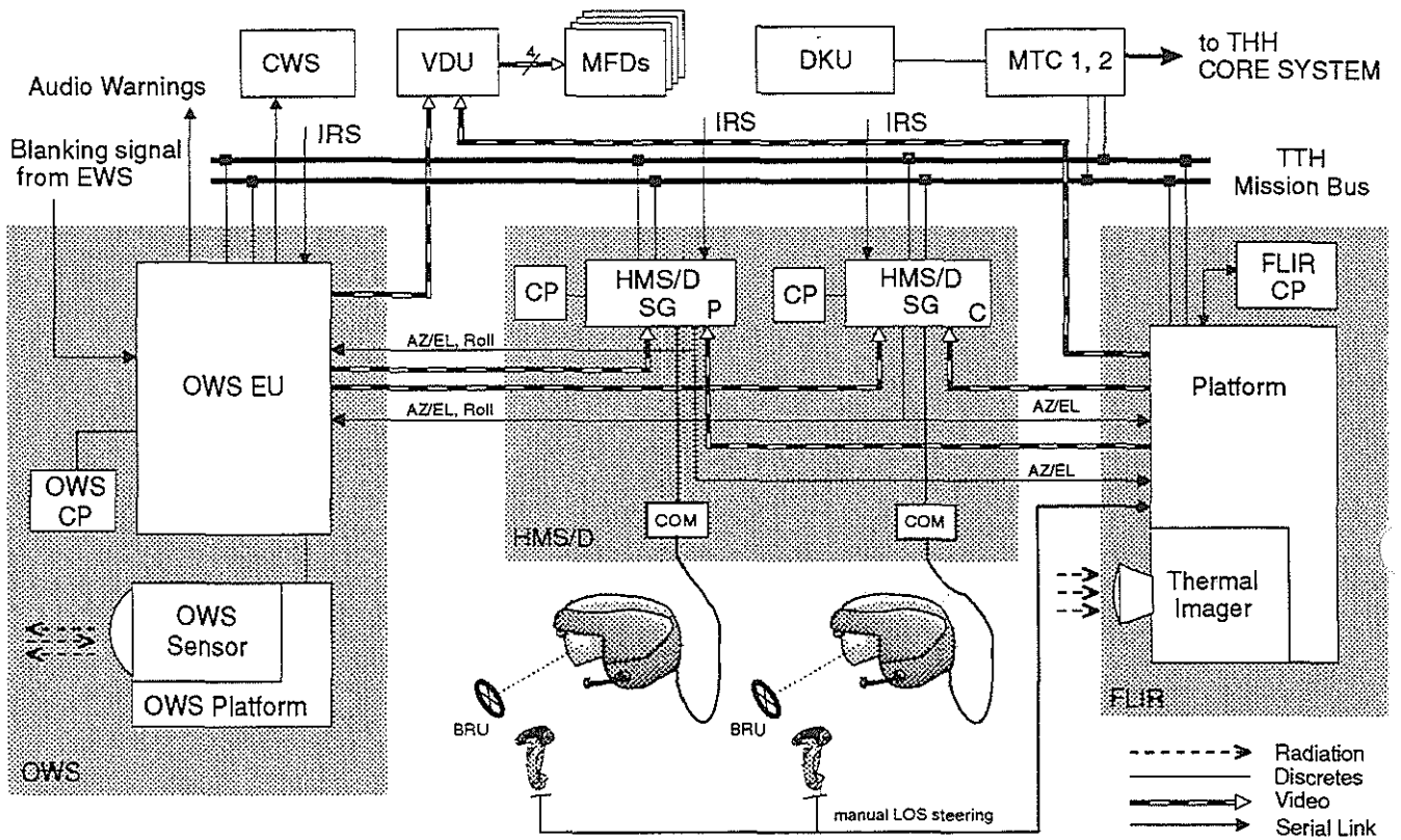
Fig. 3: System architecture of the VSA
