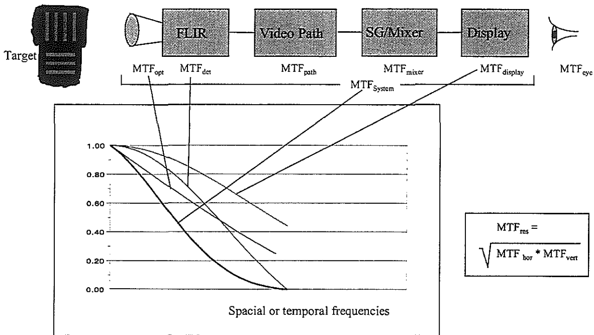
Fig. 4: Principle of the video path and the system MTF
