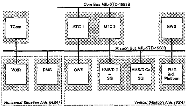
Fig. 2: Overall block diagram of the MFA in the NH90 TTH
