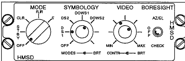
Fig. 8: The Bi-HMS/D control panel
