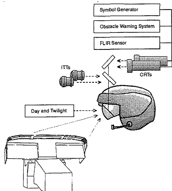
Fig. 12: Optical path of the HMD
