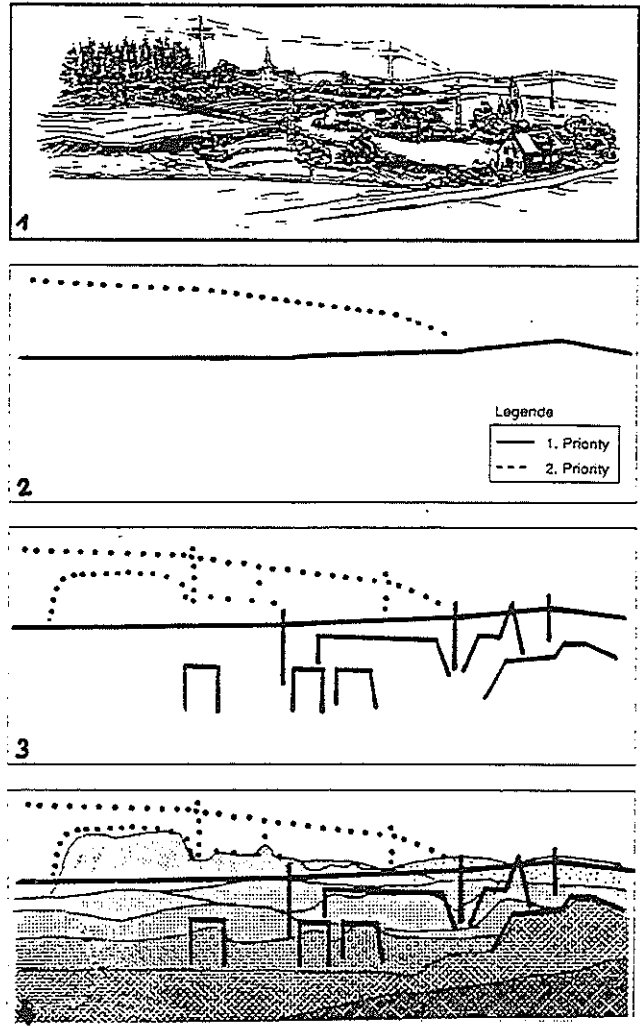
Fig. 14: 1) Outside view with eyes, FLIR or IIT 2) WIRE mode on HMD shows only wires 3) WIRE&TREE mode 4) VIDEO mode with WIRE&TREE symbology
