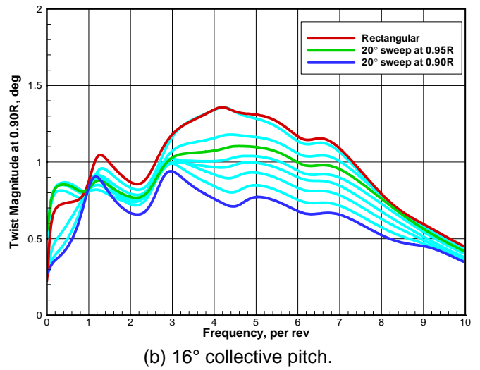
Figure 7. Active-twist frequency response for 20° sweep at various radial initiation points.
