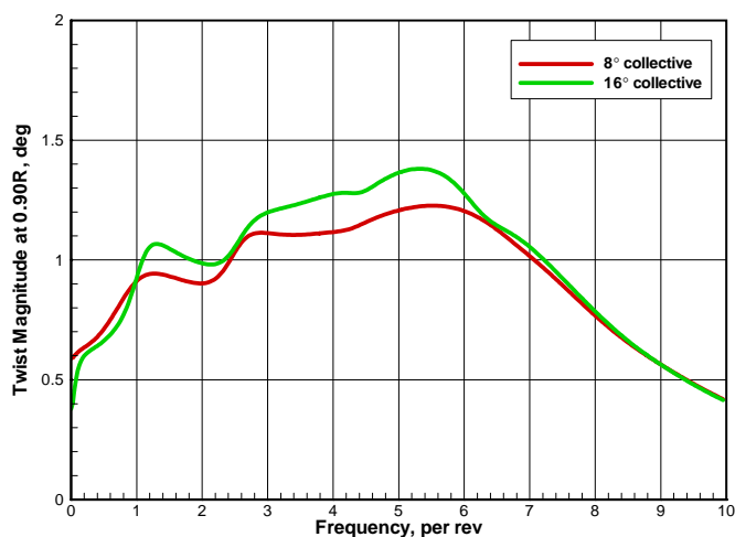
Figure 5. Effect of collective pitch variation on AATR response. Hovering flight using free wake inflow model.
