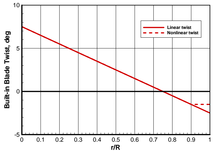
Figure 3. Blade twist definition. Linear blade twist is -10^\circ . For nonlinear twist, the twist at the nonlinear twist initiation point is extended to the tip.
