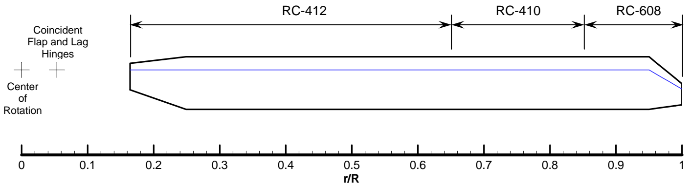
Figure 1. AATR baseline aerodynamic design planform and airfoil distribution. Blue line identifies blade quarter-chord.
