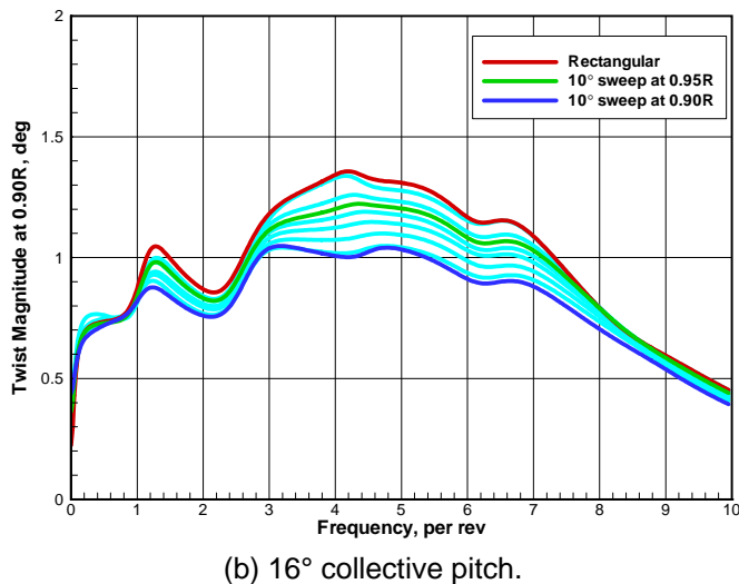
Figure 6. Active-twist frequency response for 10° sweep at various radial initiation points.
