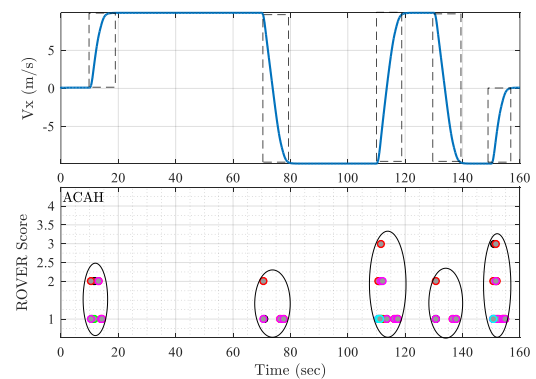
Figure 12. Multi- ROVER detection results of the ACAH Baseline
