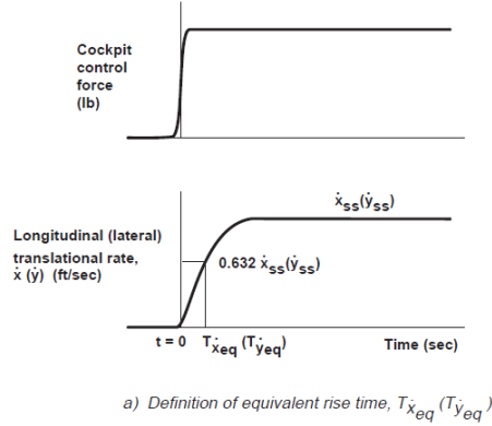
Figure 7. Definition of equivalent rise time (from ADS-33 10 )
