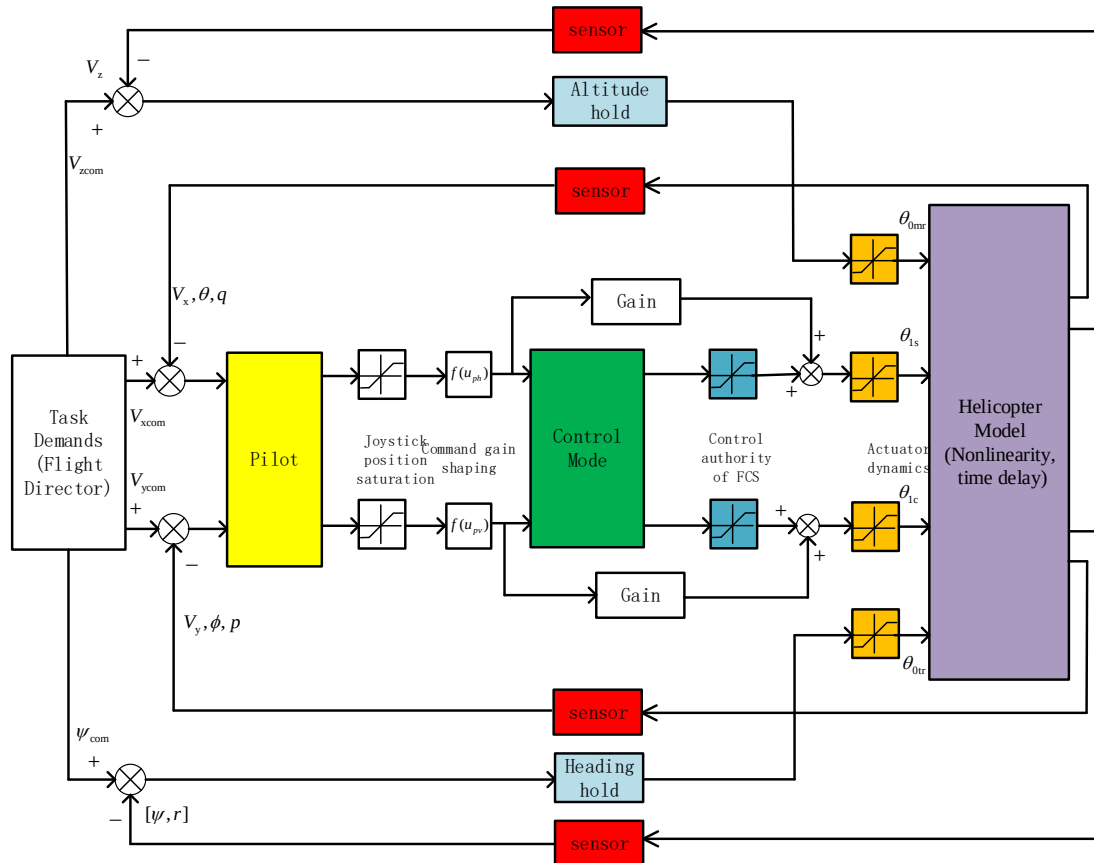
Figure 1 Structure of the pilot vehicle system
