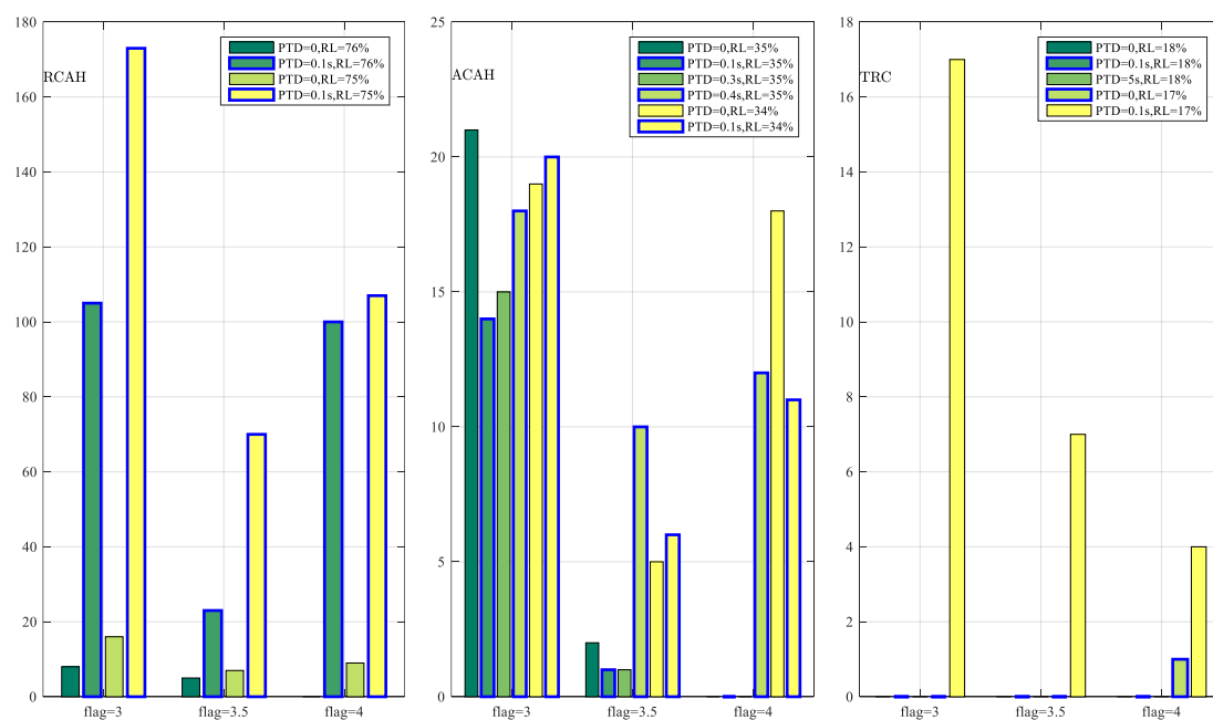
Figure 25. Multi-axis Rover detection results of sensitivity to actuator rate limit and pilot time delay
