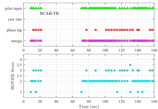
Figure 20. Single-axis ROVER detection results of RCAH mode when PTD=0.2s
