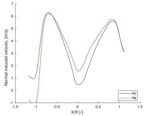
(b) Wind-on at \mu = 0.0473 and \beta = 0^\circ
