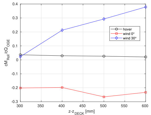
(f) Roll moment coefficient, vertical landing
