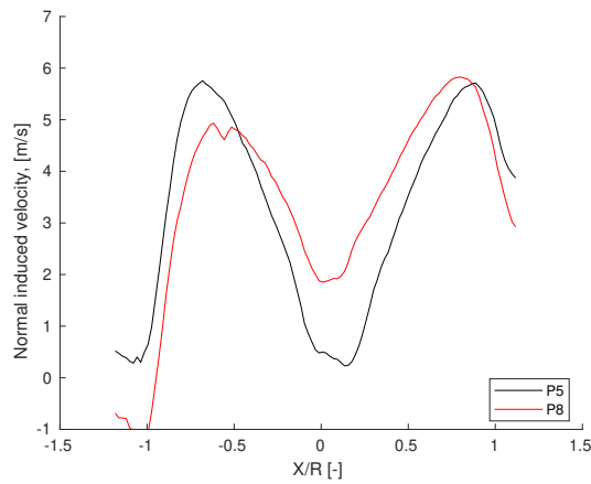
(c) Wind-on at \mu = 0.0473 and \beta = 30^\circ
