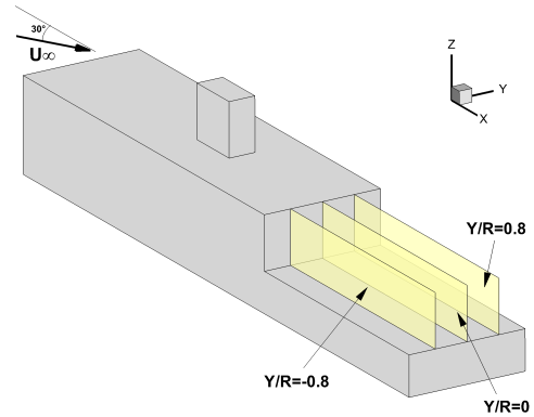
Figure 4: Position of the PIV investigation planes.
