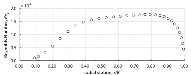
Figure 2. Approximate span-wise Reynolds number distribution for the MH rotor in the Martian atmosphere, from Koning et al. 4
