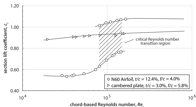
Figure 6. Variation of section lift coefficient with Reynolds number at constant angle of attack, reproduced from Hoerner 7
