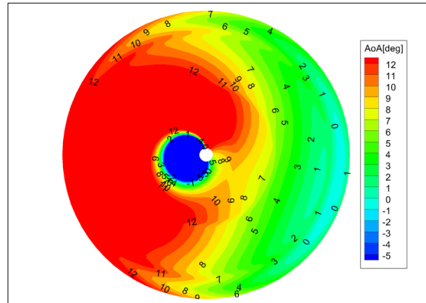
(a) front rotor
