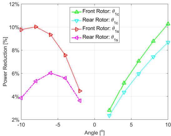
Figure 10 The effect of the cyclic pitch angles on the power reduction.
