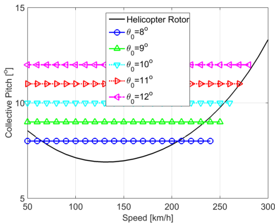
Figure 11 Variable collective pitch with forward speed.
