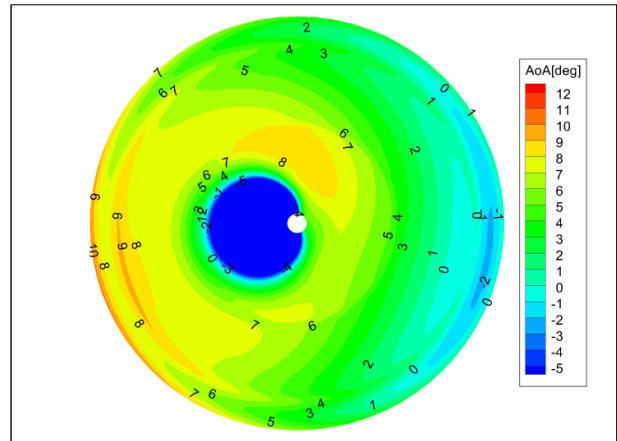
(a) helicopter rotor
