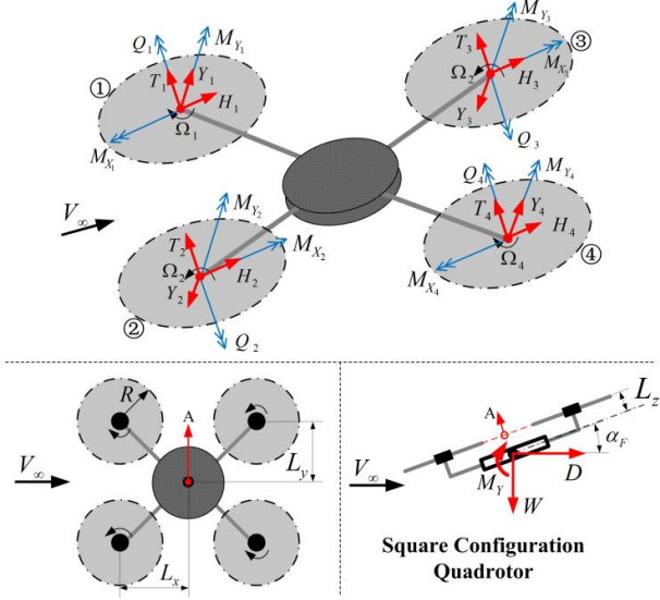
Figure 1 Forces and moment on the fuselage.
