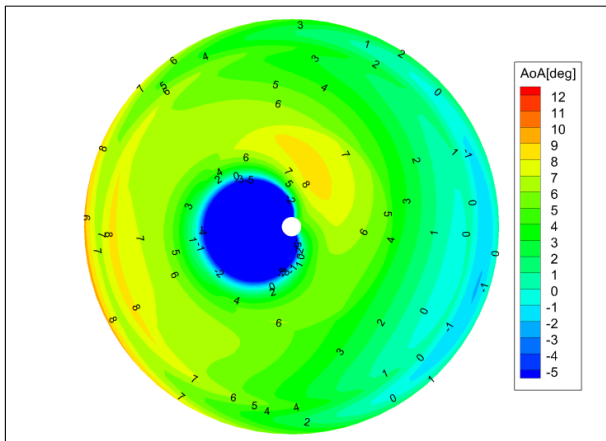
(a) front rotor
