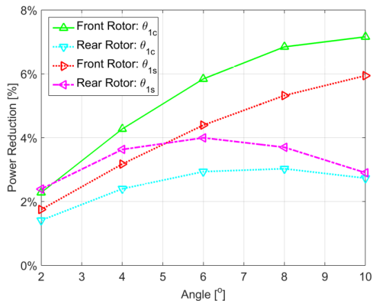
Figure 23 Power reduction by cyclic pitch control at a speed of 150km/h.
