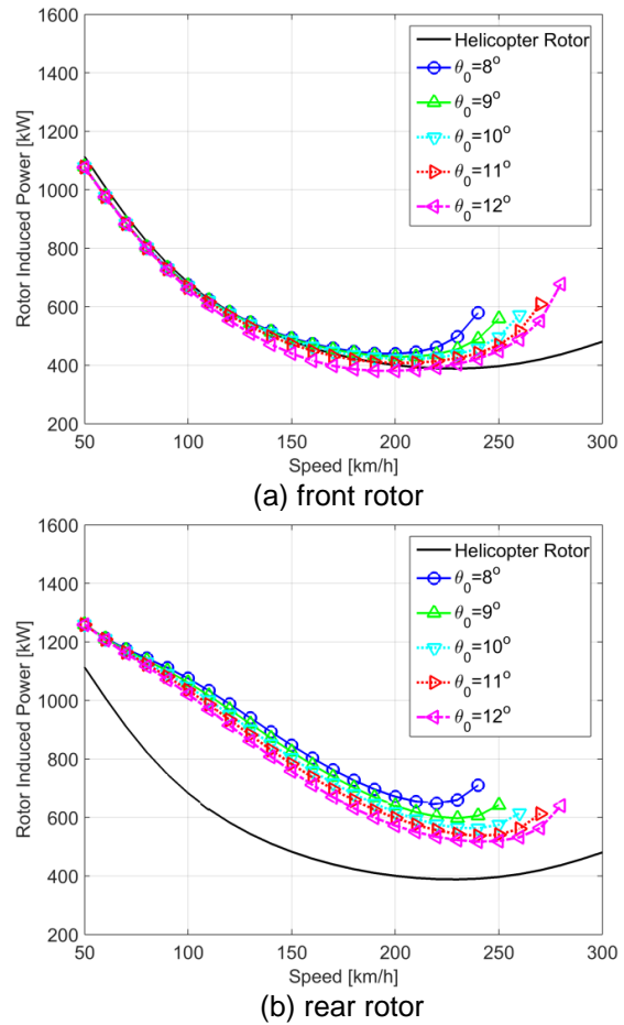
Figure 21 Rotor induced power with forward speed for different prescribed collective angles.
