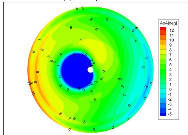
(b) front quadrotor
