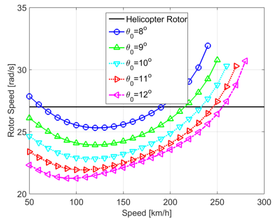
(a) front rotor
