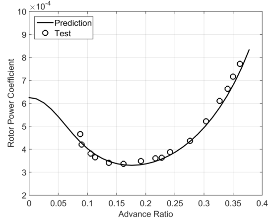
Figure 2 Comparison of predictions with flight test data.
