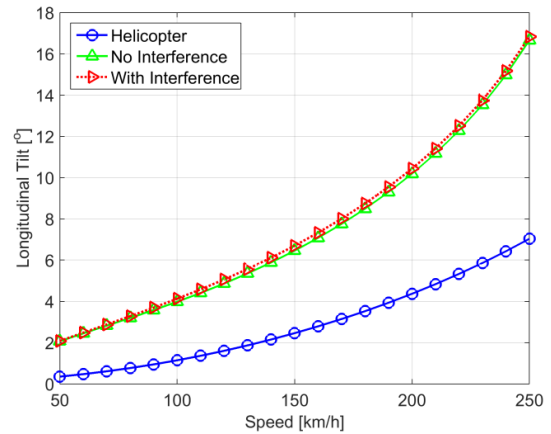
Figure 4 Longitudinal tilt with forward speed.
