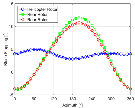
Figure 9 Steady blade flapping.
