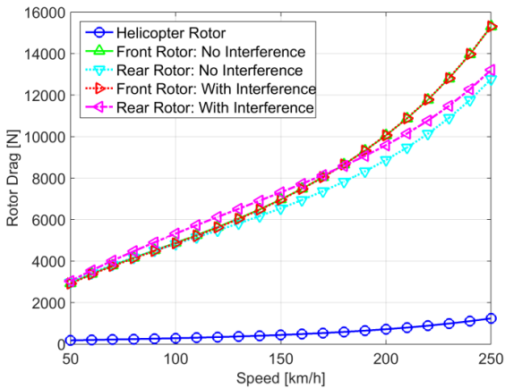
Figure 6 Rotor drag with forward speed.
