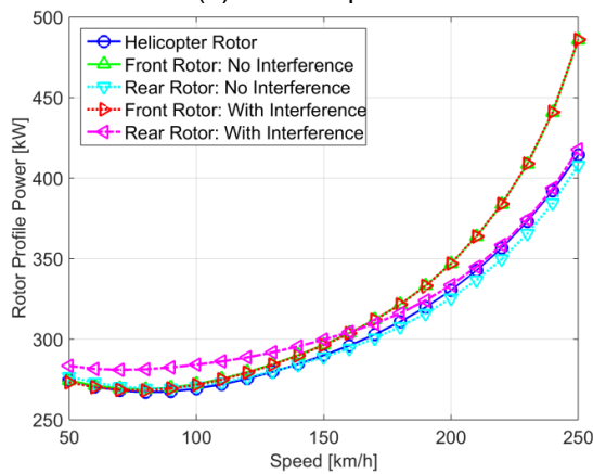
(b) profile power
