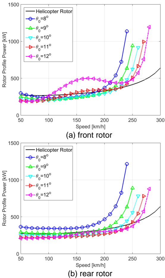
Figure 20 Rotor profile power with forward speed for different prescribed collective angles.
