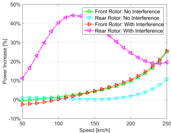
(b) power increase
