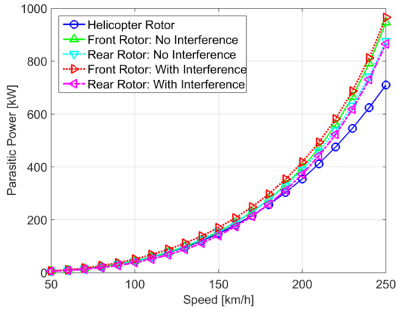
Figure 5 Parasitic power with forward speed.
