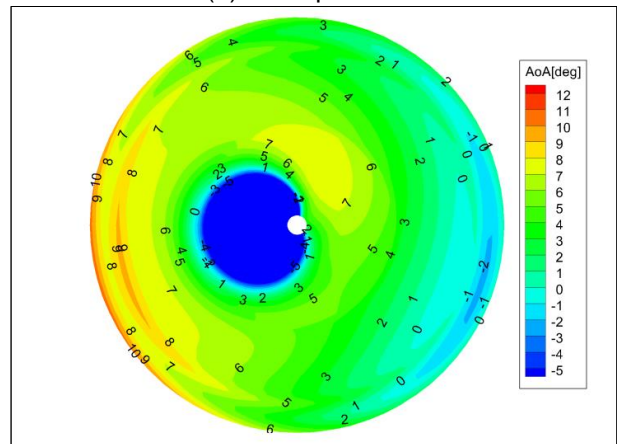
(c) rear quadrotor
