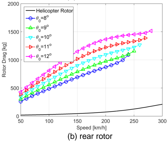
Figure 14 Rotor drag with forward speed for different prescribed collective angles.
