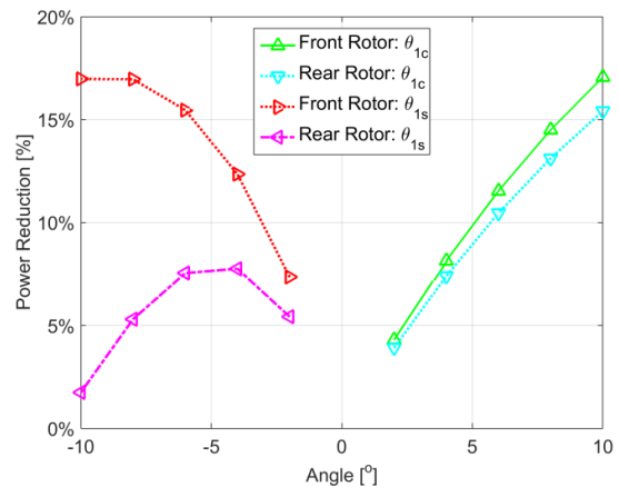
Figure 22 Power reduction by cyclic pitch control at a speed of 250km/h.
