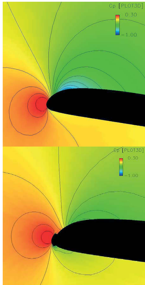
Figure 10. Pressure Distribution of Clean and Iced Rotor at r/R = 0.72 at Same Pitch
