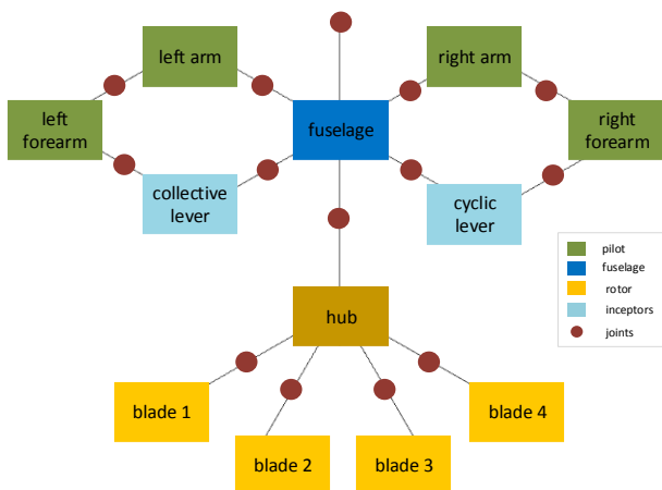
Figure 3. Pilot-Fuselage-Rotor multibody model
