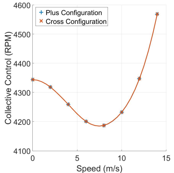
Fig. 8: Collective Control versus Flight Speed
