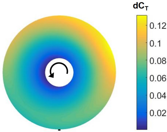
Fig. 9: Thrust Distribution over Front Rotor (Plus Configuration) at 5 m/s flight speed
