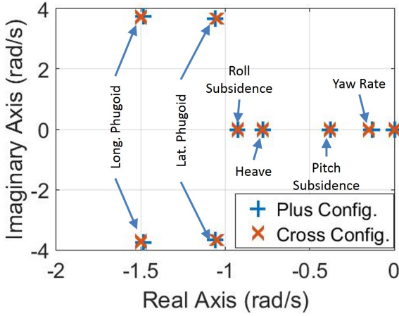
(b) Poles at 10 m/s
