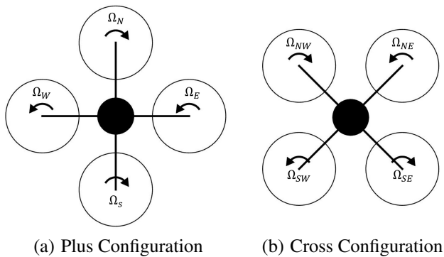
Fig. 1: Quadrotor Flight Configurations
