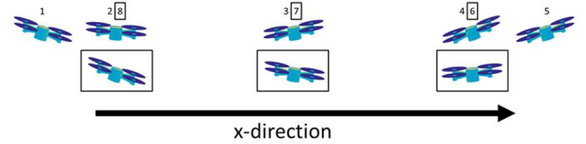
Fig. 18: Phugoid mode in hover, return segment offset vertically (shown in rectangular boxes)
