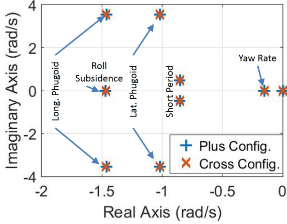
(a) Poles at 5 m/s
