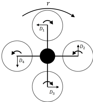
Fig. 17: Yaw Rate Mode
