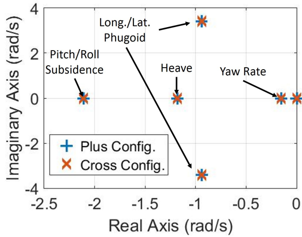
Fig. 19: Hover Poles of Plus and Cross Configuration
