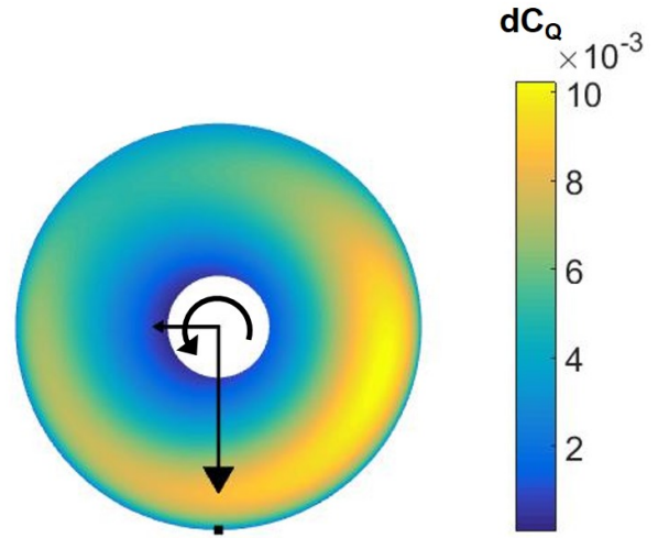
Fig. 11: Torque Distribution on front rotor (Plus Configuration) at 5 m/s flight speed
