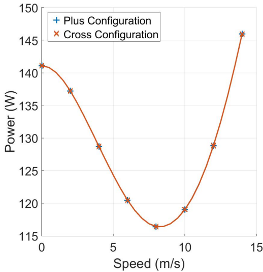
Fig. 14: Power Requirements for quadcopters
