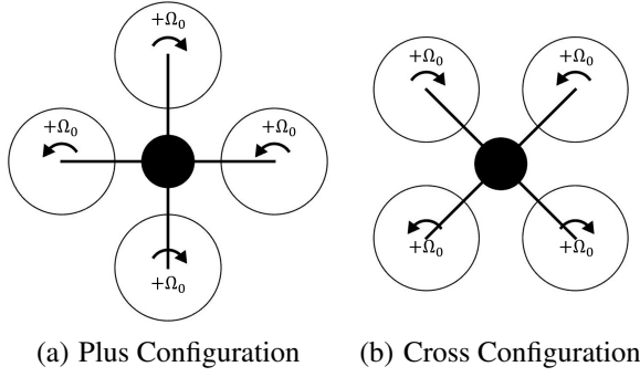
Fig. 2: Collective Control ( \Omega_0 )
