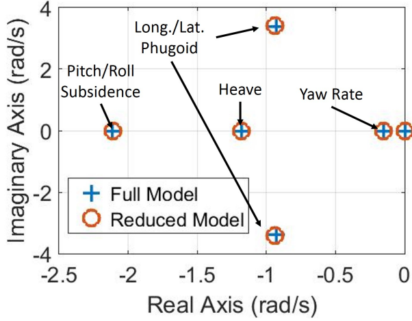
Fig. 16: Rigid body pole locations for full and reduced models (Plus configuration)
