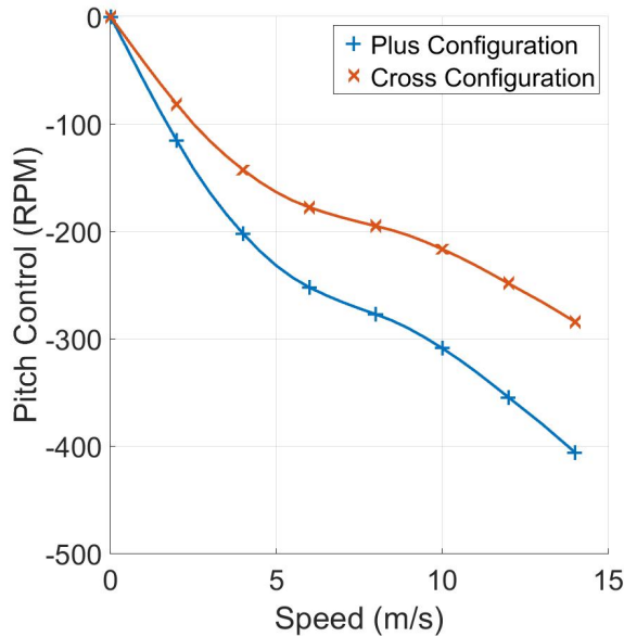
Fig. 10: Pitch Control versus Flight Speed
