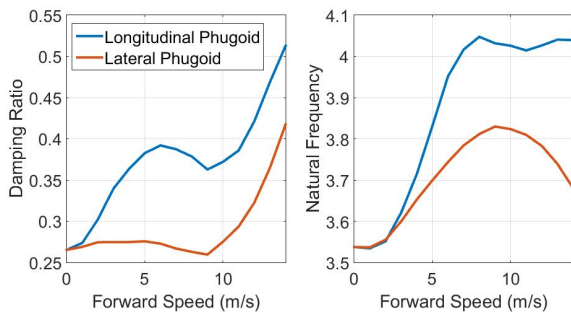
Fig. 20: Damping Ratio and Natural Frequency of the longitudinal and lateral phugoid modes in forward flight
