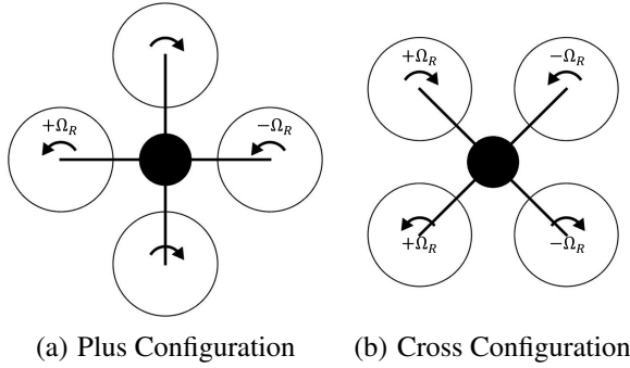
Fig. 4: Roll Control ( \Omega_R )
