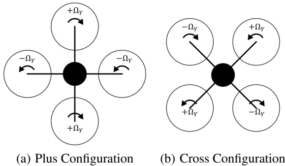
Fig. 5: Yaw Control ( \Omega_Y )
