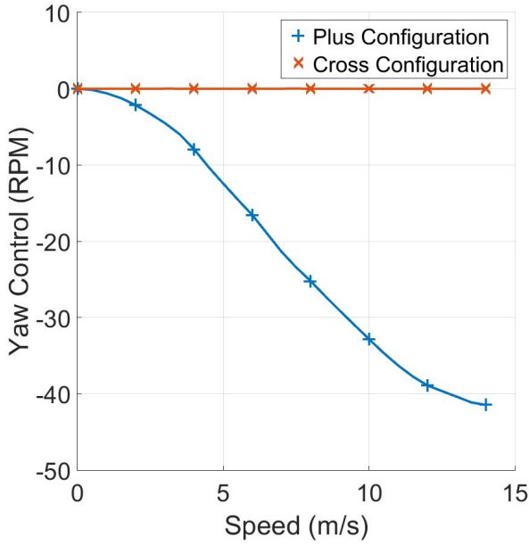
Fig. 13: Yaw Control versus Flight Speed
