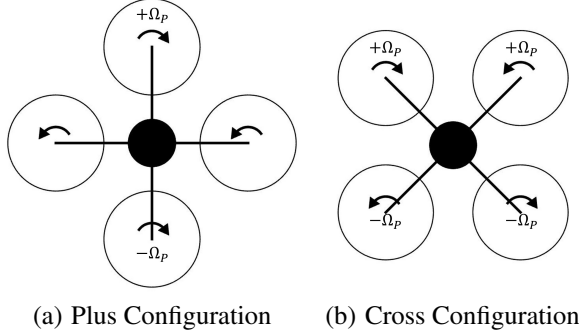
Fig. 3: Pitch Control ( \Omega_P )
