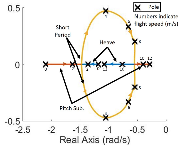
Fig. 22: Pitch Subsidence and Heave Modes
