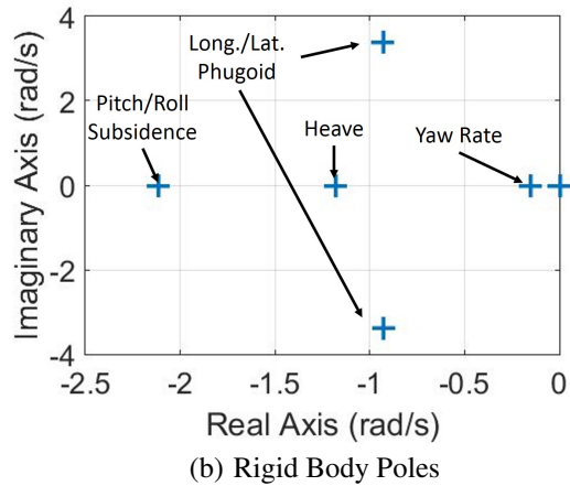
Fig. 15: Locations of the poles of the quadcopter in hover (Plus configuration)
