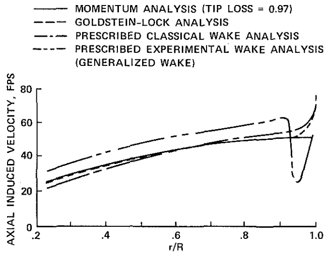
Figure 8. Comparison of induced velocities calculated from momentum theory and three prescribed-wake analyses (from Ref. 56).
