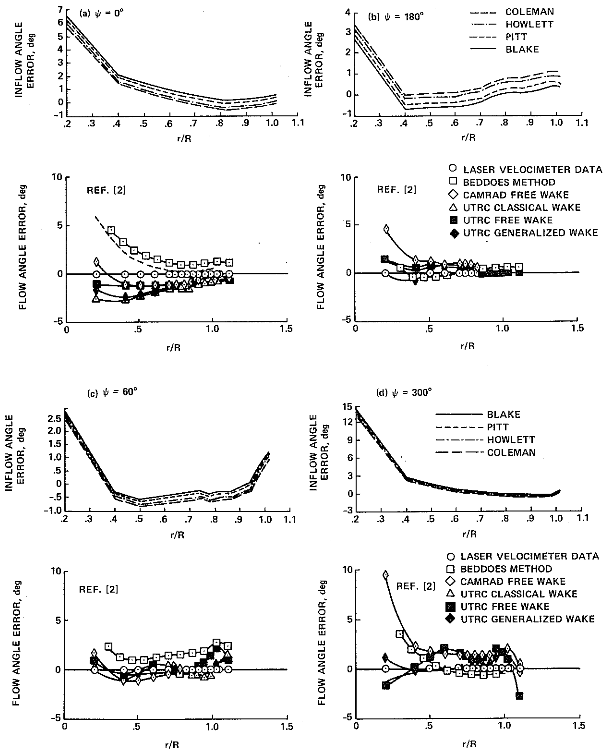
Figure 36. Comparison of inflow-angle errors calculated from simple first-harmonic inflow models with those from wake models evaluated in Ref. 2, \mu = 0.15 . (a) \psi = 0^\circ . (b) \psi = 180^\circ . (c) \psi = 60^\circ . (d) \psi = 300^\circ .
