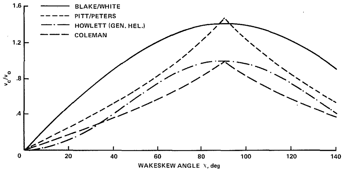
Figure 15. Comparison of v_c/v_0 for several inflow models.
