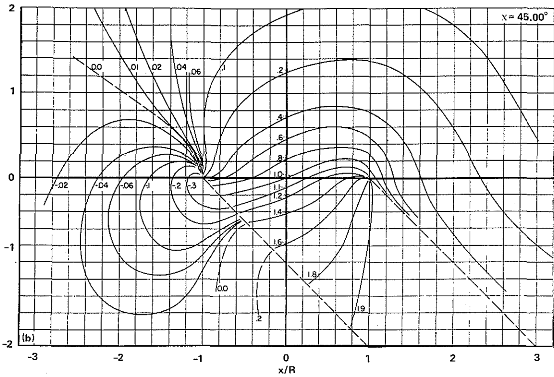
Figure 14. Lines of constant values of isoinduced velocity ratio v/v_0 in longitudinal plane of symmetry for several wake skew angles (from Ref. 16). (a) \chi = 26.56^\circ . (b) \chi = 45^\circ .
