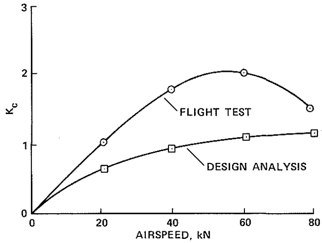
Figure 23. Comparison of K_c values used in the design analysis and determined from flight test (from Ref. 25).
