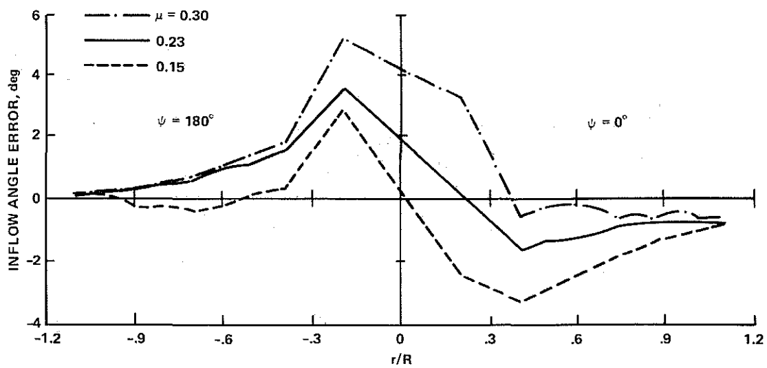
Figure 41. Induced inflow errors generated from Takahashi model in the longitudinal plane of symmetry for the three advance ratios tested in Ref. 1.
