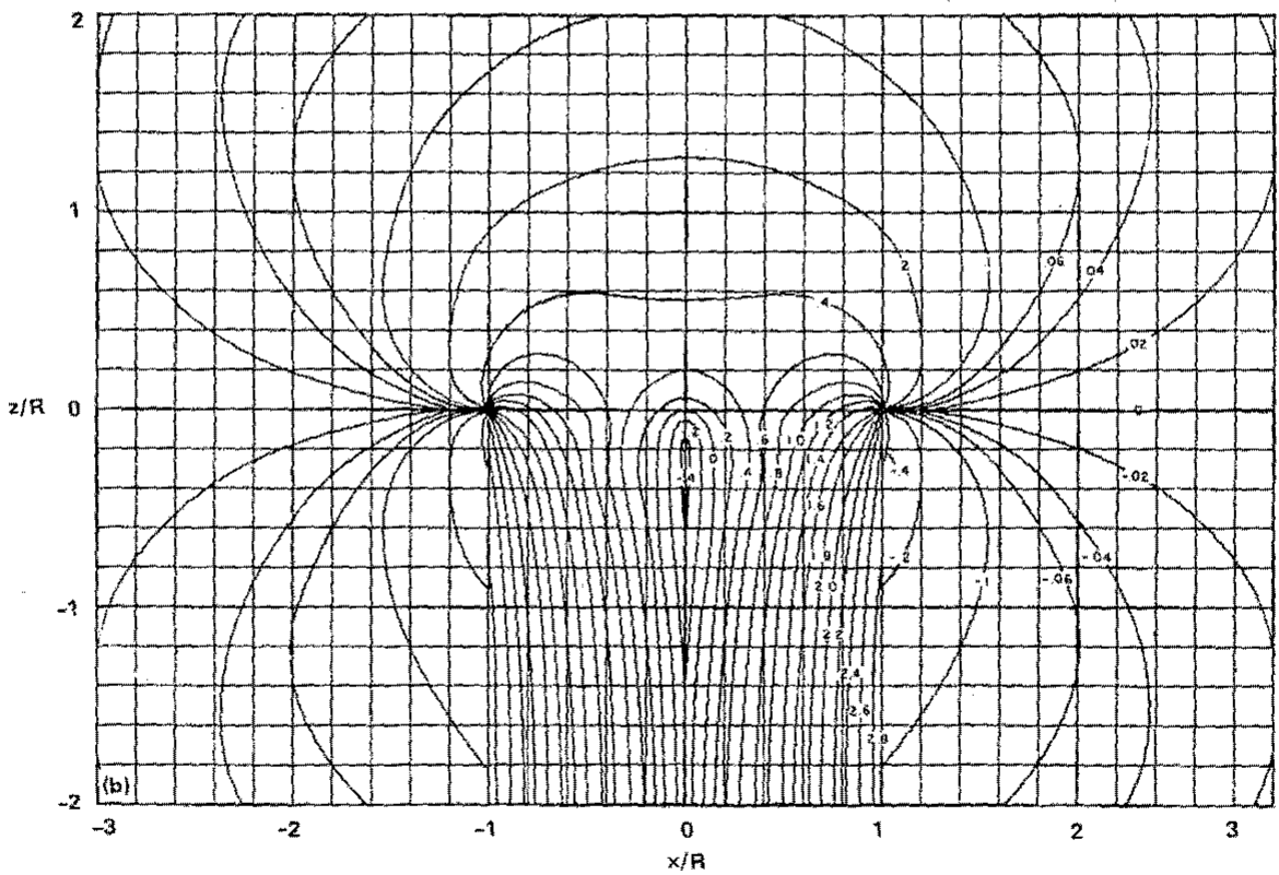
Figure 9. Contours of induced-velocity ratio v/v_0 in the longitudinal plane of the rotor for two different disk loadings at \chi = 0^\circ (from Ref. 16).
