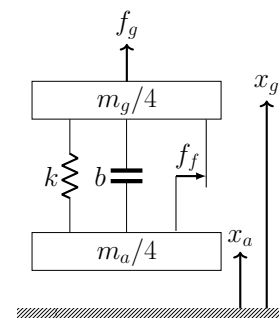
Figure 9: Quarter H/C model
