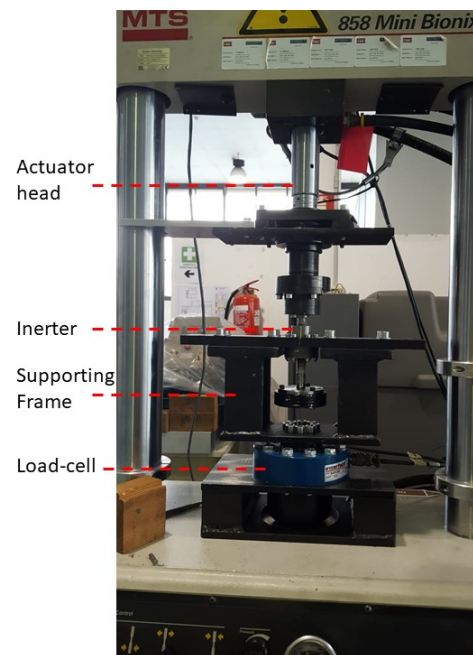
Figure 5: Test set-up
