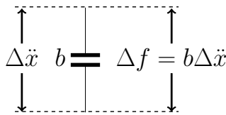
Figure 2: The inerter produces an internal force proportional to the relative acceleration.
