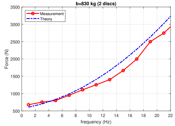
Figure 7: Force Measurement of 2 disc configuration and comparison with theory (linear inerter+friction)
