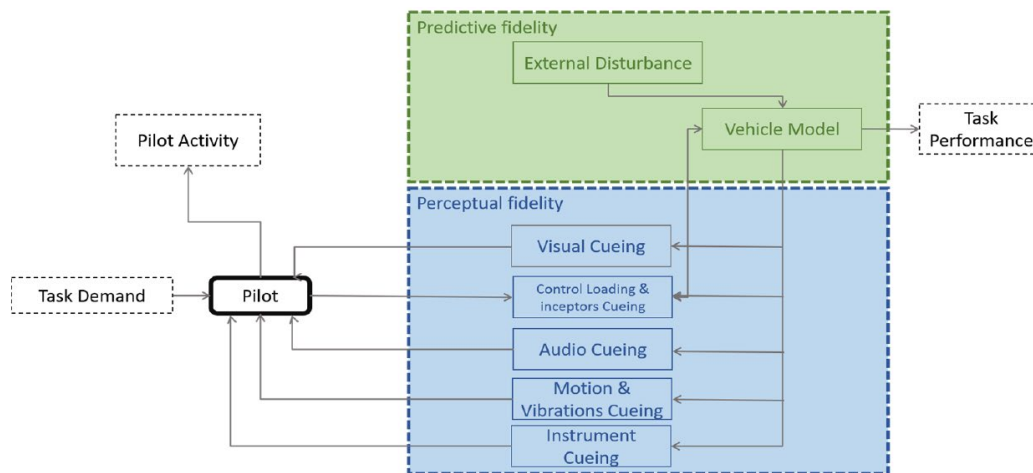
Figure 1 The flight model and simulator cueing systems as elements of the integrated flight simulation.
