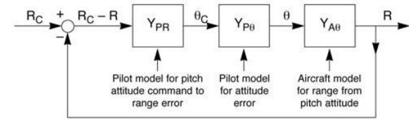
Figure 5 Closed-loop control of aircraft range.
