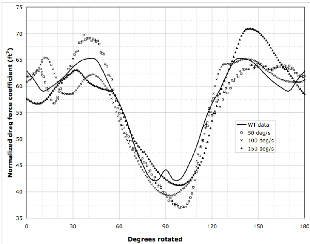
Figure 8 Comparison of drag force ( C_{DA} ) between stationary WT data and moving-body CFD results ( \alpha = 0^\circ )
