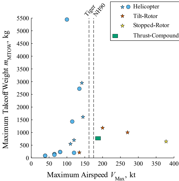
Figure 1-1: Overview of currently available VTOL-UAVs and the expected solution area of the FaUSt-Demonstrator (commercial product (circle), demonstrator or prototype (star))
