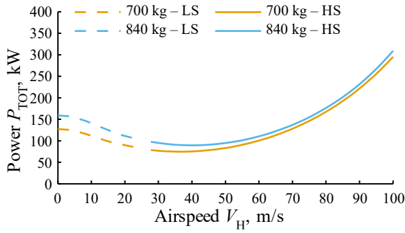
Figure 4-4: Power distribution in forward flight for different flight masses (LS – low-speed, HS – high-speed)
