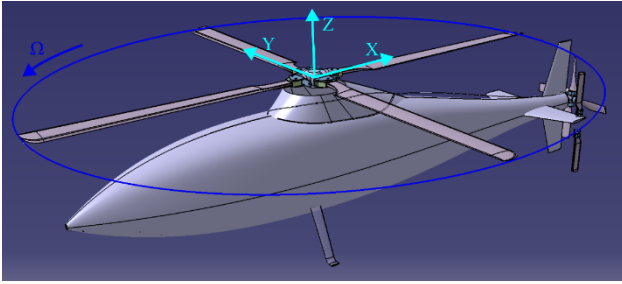
Figure 3-4: Concept of main rotor system
