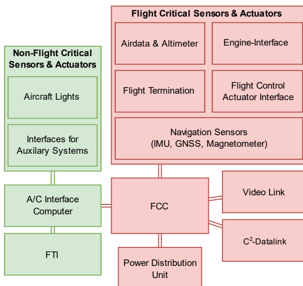
Figure 3-10: Overview of the avionics with flight critical parts in red and non-flight critical in green
