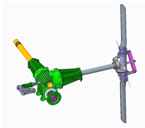
Figure 3-8: Concept of the tail rotor control system
