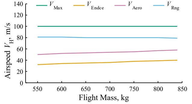
Figure 4-9: Characteristic velocities for different flight masses
