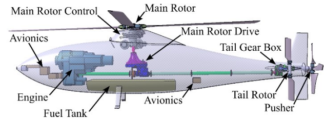
Figure 3-1: External and internal arrangement of the system and subsystems
