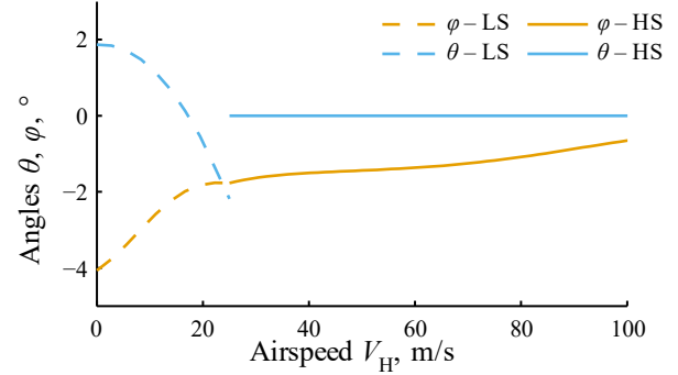
Figure 4-2: Trim values of the pitch and roll angle \theta and \varphi (LS – low-speed, HS – high-speed)
