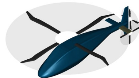
Figure 2-2: Candidate 1 - Thrust-Compound
