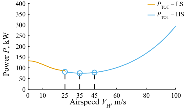
Figure 4-1: Total power curve with the test points of the maneuver flight (LS – low-speed, HS – high-speed)
