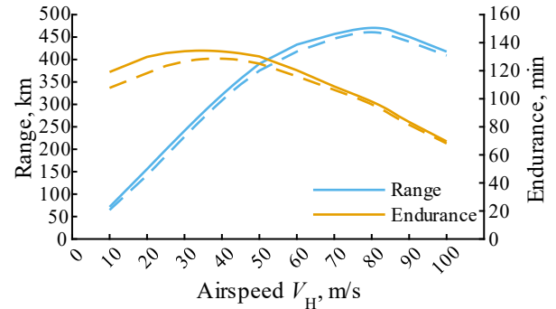
Figure 4-10: Dependence of endurance and range on airspeed (ISA sea level, 700 kg – solid, 840 kg – dashed)
