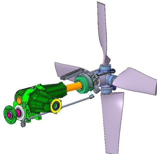
Figure 3-9: Concept of the pusher control system
