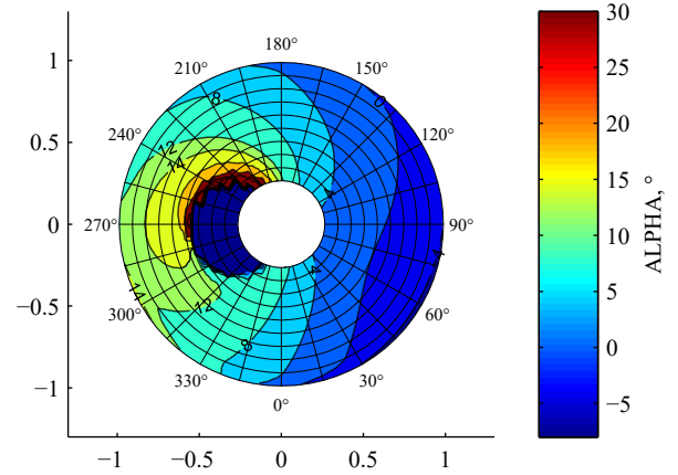
Figure 4-6: Angle of attack \alpha at 100 m/s airspeed at the rotor disk
