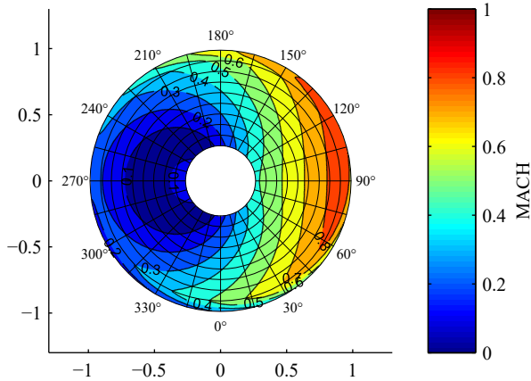
Figure 4-5: Mach number at 100 m/s airspeed at the rotor disk
