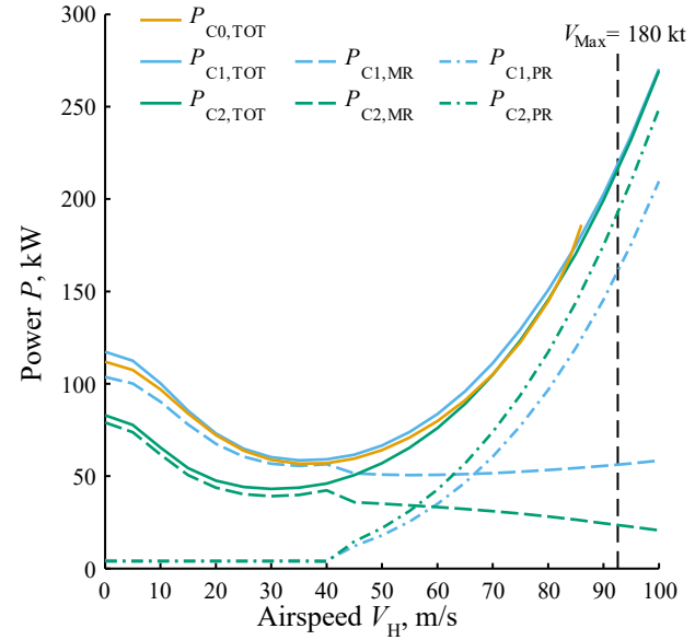
Figure 2-4: Forward flight performance of the candidates (total power ( P_{TOT} ), power main rotor ( P_{MR} ), power pusher ( P_{PR} ))
