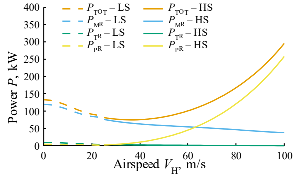
Figure 4-3: Power distribution of different components (total power ( P_{TOT} ), power main rotor ( P_{MR} ), power tail rotor ( P_{TR} ), power pusher ( P_{PR} ) / (LS – low-speed, HS – high-speed)
