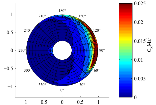
Figure 4-7: C_x Ma^2 at 100 m/s airspeed at the rotor disk
