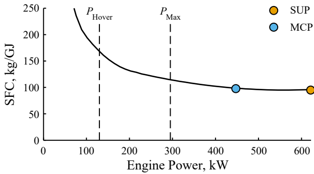
Figure 4-8: Specific Fuel Consumption (SFC) over engine power
