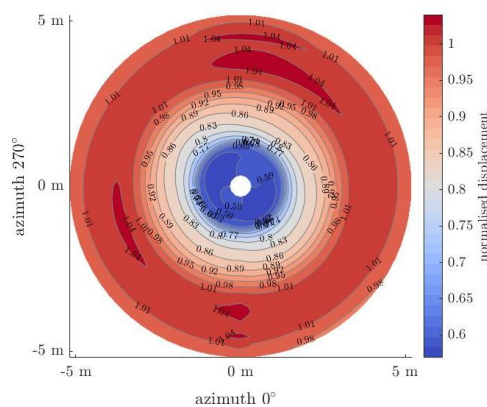
Figure 4: Typical output of stochastic model
