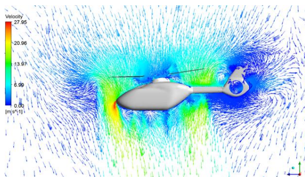
Figure 2: Downwash in hover condition at 1000 ft
