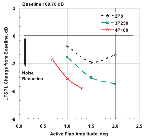
Figure 12: Effect of active flap excitation frequency and amplitude for "best" phase on LFSPL at microphone M13; \mu = 0.3 , \alpha = -9.1^\circ
