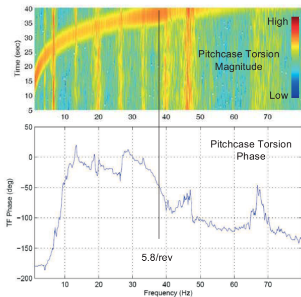
Figure 7: Pitchcase torsion magnitude (power spectral map, log scale) and phase (deg) from active flap frequency sweep; 200V collective, 0.2-80 Hz log sweep, hover, \alpha = -10^\circ , collective pitch = 4^\circ
