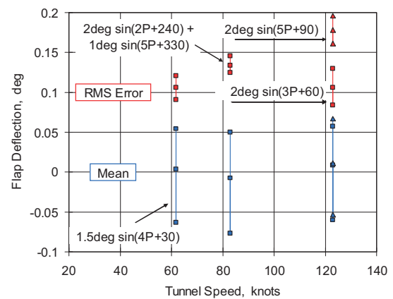
Figure 5c: Active flap mean deflection and RMS error versus speed, closed-loop flap position control with four harmonic commands
