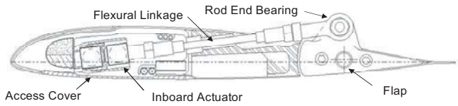
Figure 1e: SMART Blade, flap, actuator cross-section
