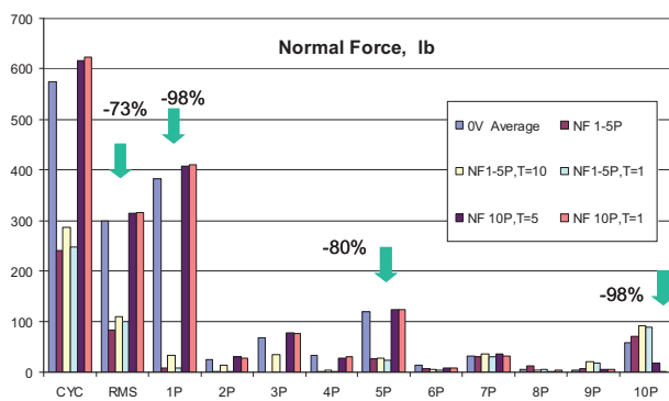
Figure 15: Vibratory hub normal force and vibration index for baseline case (0V) and closed-loop active flap control of normal force (NF); \mu = 0.3 , \alpha = -9.1^\circ
