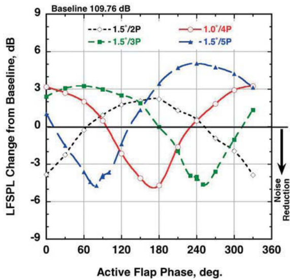
Figure 11: Effect of active flap excitation frequency and phase on LFSPL at microphone M13; \mu = 0.3 , \alpha = -9.1^\circ
