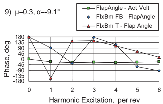
Figure 8, 9: Phase relationships for excitation at rotor speed multiples; active flap vs voltage and flexbeam flap bending and torsion vs active flap
