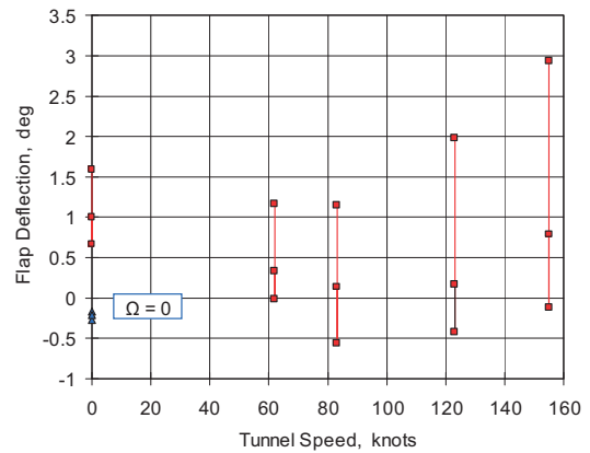
Figure 5a: Active flap deflection versus speed, open-loop flap with 0 Volt applied
