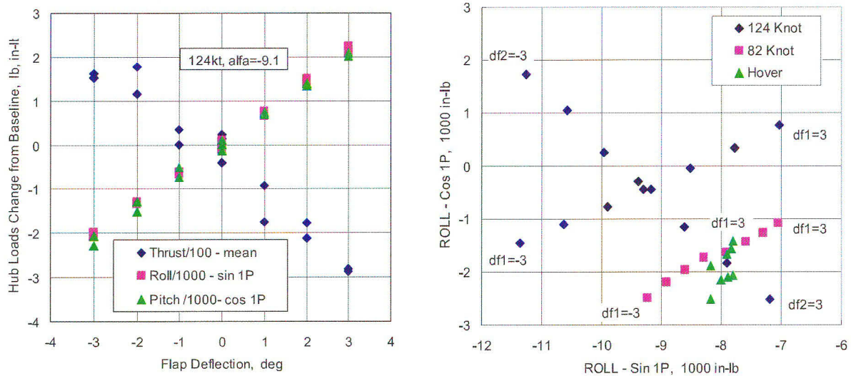
Figure 17: Rotor smoothing: hub load changes from steady inputs of -3 to +3 deg on a single active flap. a) thrust (mean), roll moment (sin1P), and pitch moment (cos1P) relative to baseline with flap 1; \mu = 0.3 , \alpha = -9.1^\circ ; b) roll moment (1P) with flap 1 or flap 2 (df1, df2); \mu = 0 , \alpha = -10^\circ ; \mu = 0.2 , \alpha = 2^\circ ; \mu = 0.3 , \alpha = -9.1^\circ
