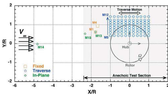
b) Microphone layout (top view)
