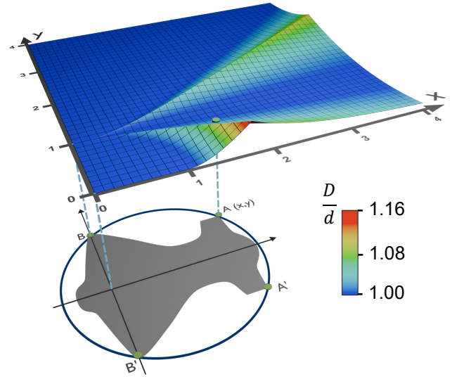
Figure 9: Ratio of the smallest enclosing circle diameter to the largest overall dimension, as a function of the normalized coordinates of point A .
