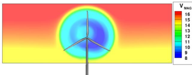
a) Velocity field
