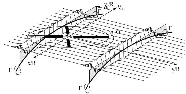
Figure 10 Schematic of the helicopter rotor – wind turbine wake vortex model
