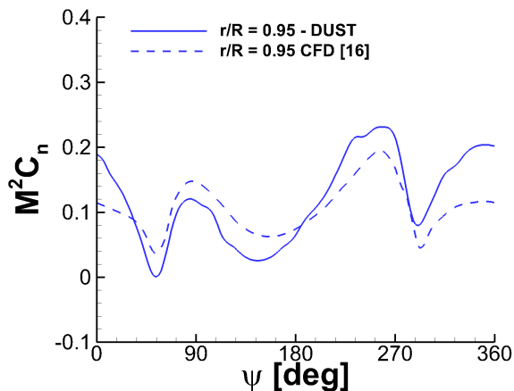
Figure 7: Comparison of the time histories of the non-dimensional normal force M^2C_n on the propeller blade in conversion flight condition at r/R = 0.95 , \theta_N = 75^\circ , V_\infty = 40 kts, \Omega = 589 RPM (from [14]).
