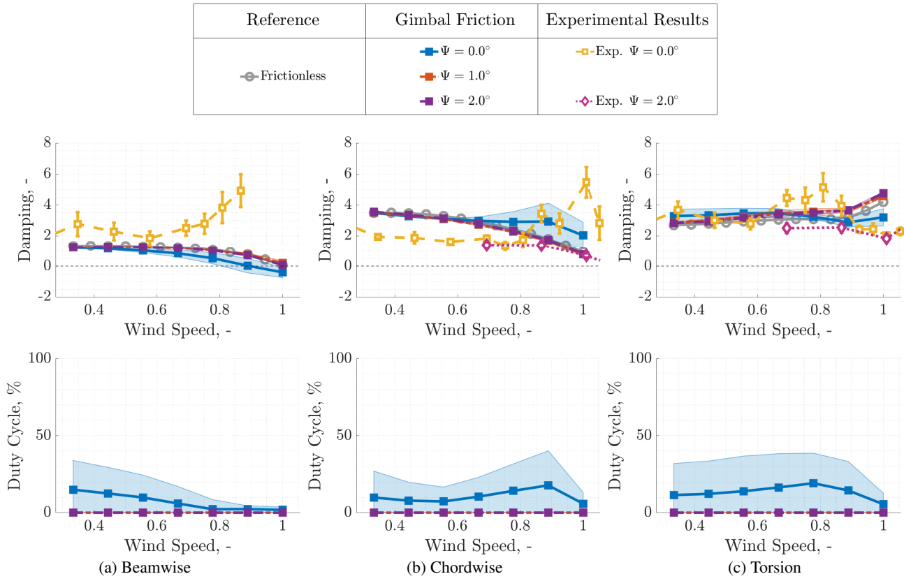
Figure 9: Effect of gimbal spherical friction on structural mode damping.
