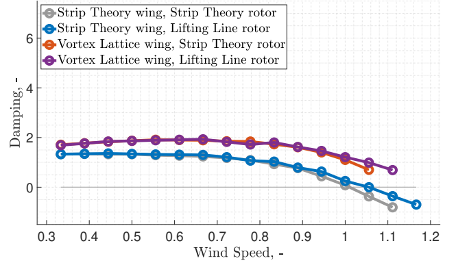
(a) Beamwise mode damping.
