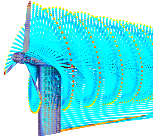
Figure 2: Example of the DUST aerodynamic surfaces and wake on the ATTILA model.
