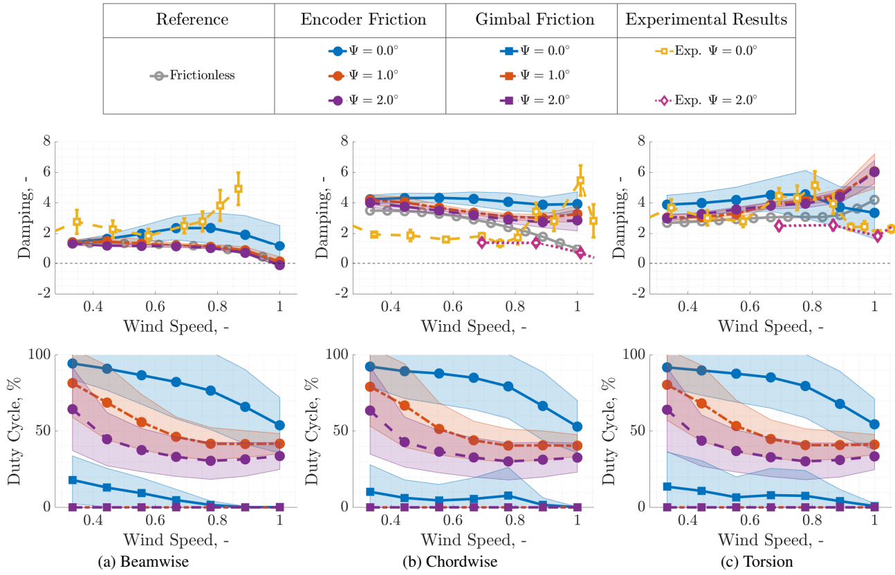
Figure 10: Effect of combined gimbal spherical friction and encoder friction on structural mode damping.
