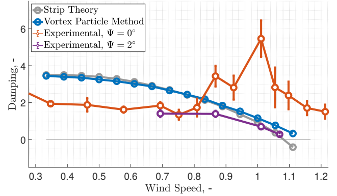
(b) Chordwise mode damping.
