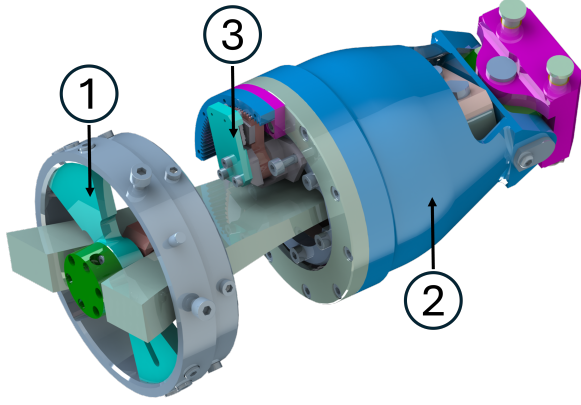
Figure 6: CAD model of the pitch bearings (inner, 1, and outer, 2) and encoder (3).
