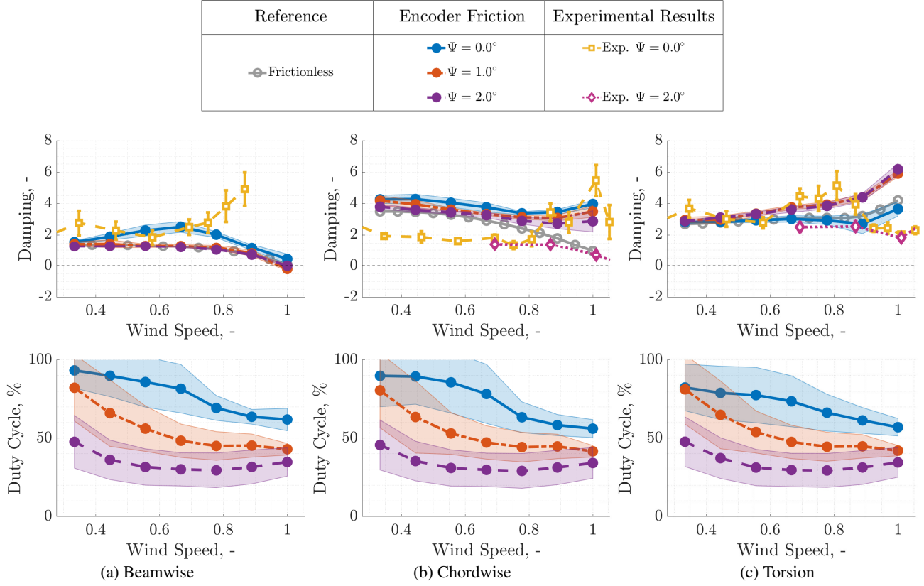
Figure 7: Effect of pitch encoder friction on structural mode damping.
