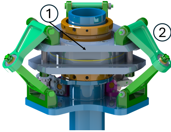
Figure 8: CAD model of the gimbal joint assembly (yoke, 1, and compasses, 2).
