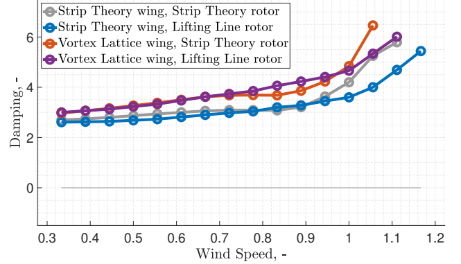
(c) Torsion mode damping.
