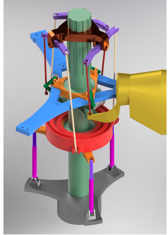
Figure 4: Layout of the XV-15 rotor control chain.
