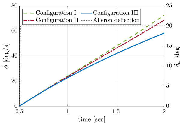
Figure 11: Comparison of the roll rate evolution.
