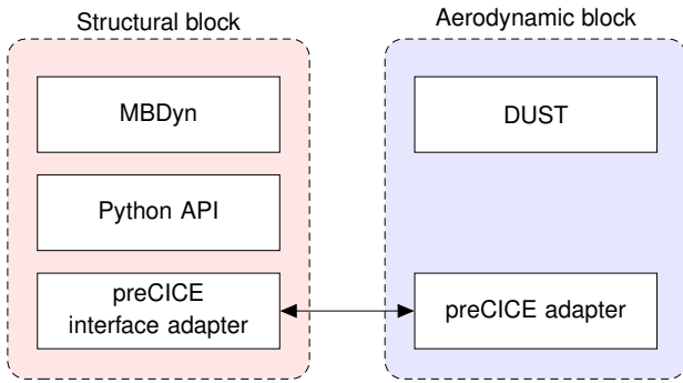
Figure 1: Communication managed through the two solvers adapters
