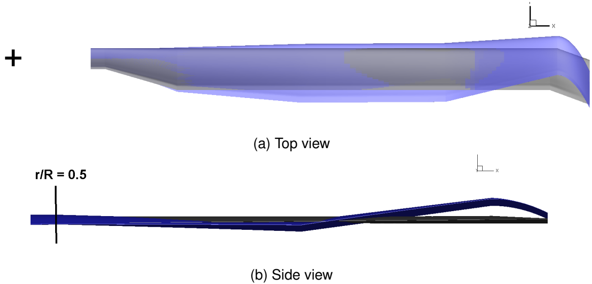
Figure 4: Comparison between the baseline (grey) and forward flight optimised (blue) planform shapes for the AH-64A rotor blade in forward flight at C_T = 0.00903 , \mu = 0.3 .
