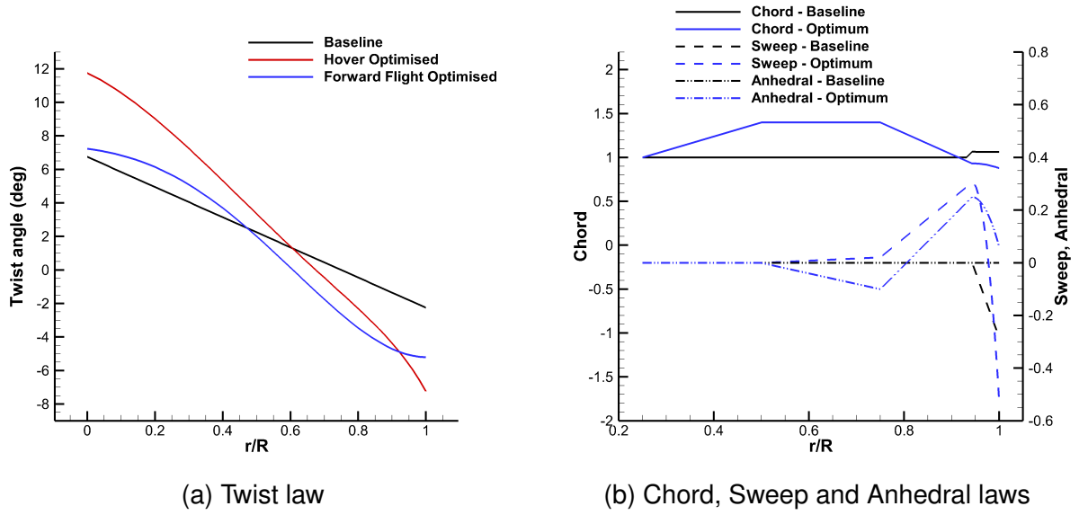
Figure 3: Comparison of baseline AH-64A and forward flight optimised geometric laws. Chord, Sweep and Anhedral values given based on a unit chord length (chord of first aerodynamic section).
