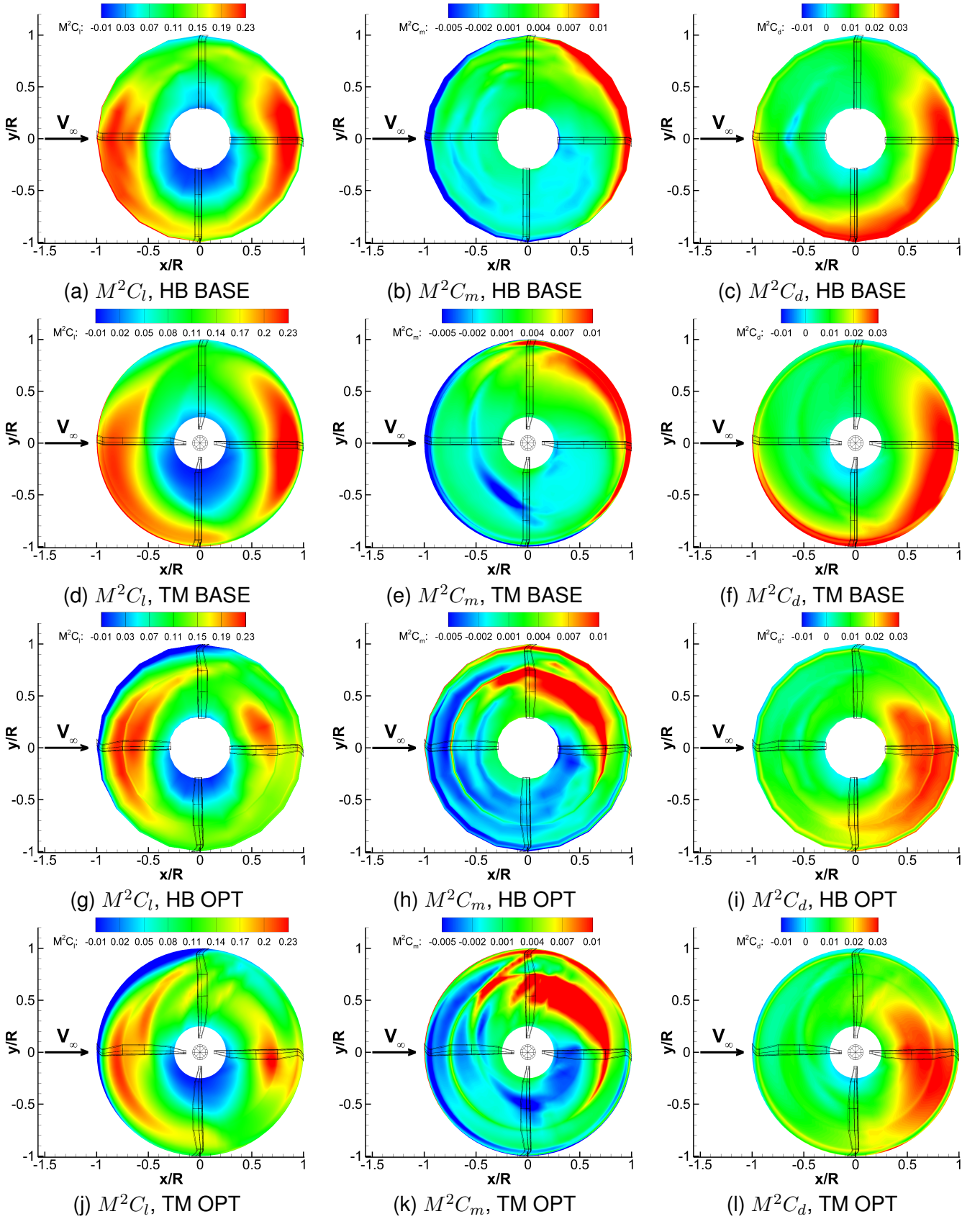
Figure 5: Comparison of the rotor disk loads for the baseline (BASE) parameterised and optimised (OPT) AH-64A rotor blades in forward flight at C_T = 0.00903 , \mu = 0.3 based on 2 mode harmonic balance (HB) and time-marching (TM) calculations.
