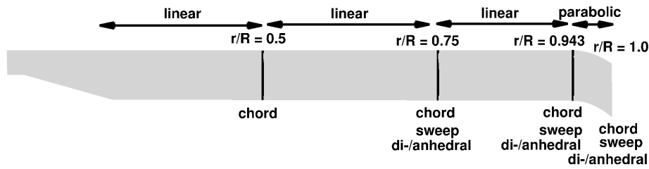
Figure 1: Blade surface parameterisation shown based on the AH-64A blade used within optimisation study.
