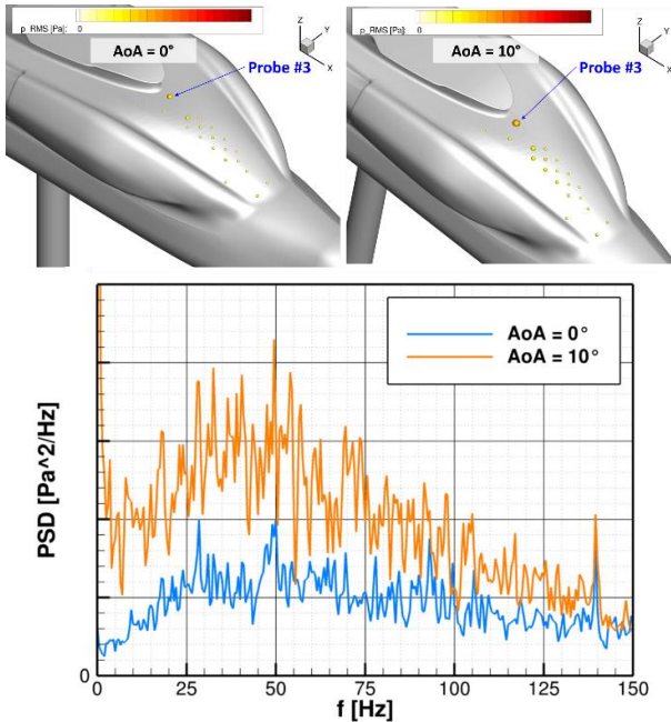
Figure 21 – Top: RMS pressure at the skin pressure sensors for AoA = 0° and 10°; the sensor sphere radii are sized and colored by RMS pressure; Bottom: PSD of static pressure at probe #3; Configuration AI_NONE, AoY = 0°, U = 40 m/s
