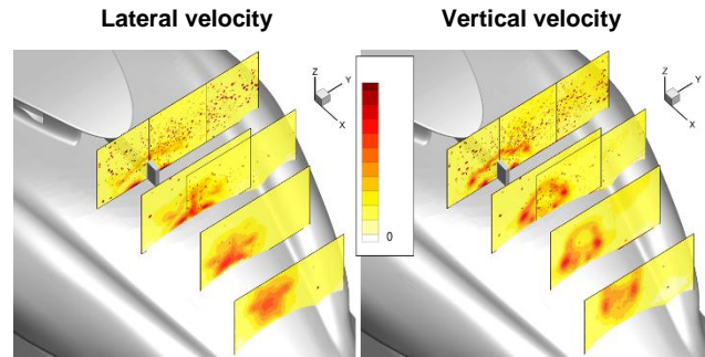
Figure 31 – RMS velocity field in the PIV planes; Configuration AI_OA1_xe3; Operating air intakes; AoA = 0°, AoY = 0°, U = 40 m/s
