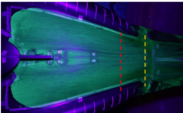
Figure 29 – Locations of the mean flow-separation for AoA = 0°; Rear-central separation in yellow; Lateral separation in red; Configuration AI_OA1_xe3; Operating air intake; AoY = 0°, U = 40 m/s
