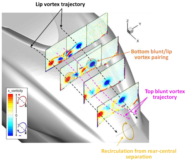
Figure 17 – Mean longitudinal vorticity in the PIV planes and interpreted vortex trajectory; Configuration AI_NONE, AoA = 0°, AoY = 0°, U = 40 m/s
