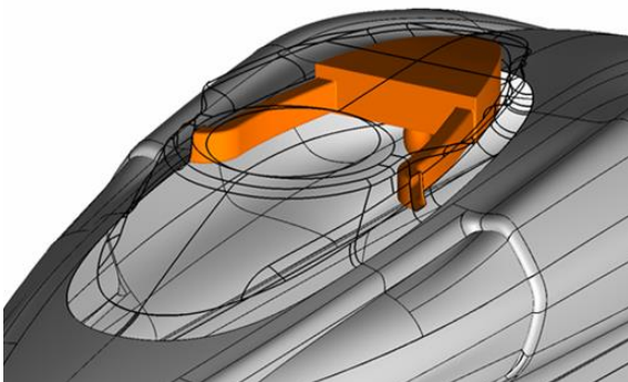
Figure 7 – Air intake #2 (AI_BU) located on the side of the pylon fairing
