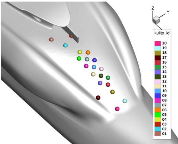
Figure 14 – Pressure-sensor implementation on the rear cowlings and associated sensor IDs
