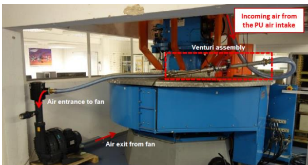
Figure 11 – General view of the PU suction installation
