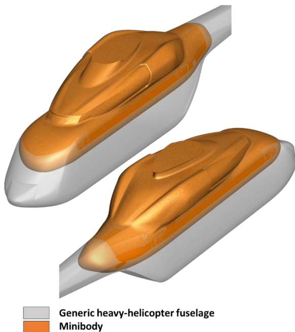
Figure 3 – Generic heavy-helicopter fuselage and associated minibody
