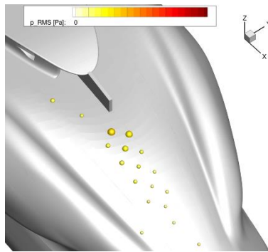
Figure 33 – RMS pressure at the skin pressure sensors for AI_OA1_xe3 configuration at \text{AoY} = +6^\circ ; the sensor sphere radii are sized and colored by RMS pressure ; \text{AoA} = 0^\circ , U = 40 \text{ m/s}
