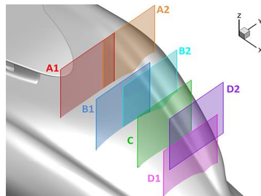
Figure 12 – Overview of the seven PIV windows considered during the campaign, for zero angle of attack and zero yaw
