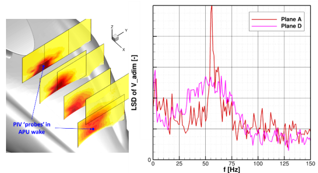
Figure 28 – Left: RMS lateral velocity field in the PIV planes with probes located in the APU wake; Right: Linear spectral density (LSD) of the lateral velocity component in APU wake; Configuration AI_REF, operating APU, AoA = 0^\circ , AoY = 0^\circ , U = 40 m/s
