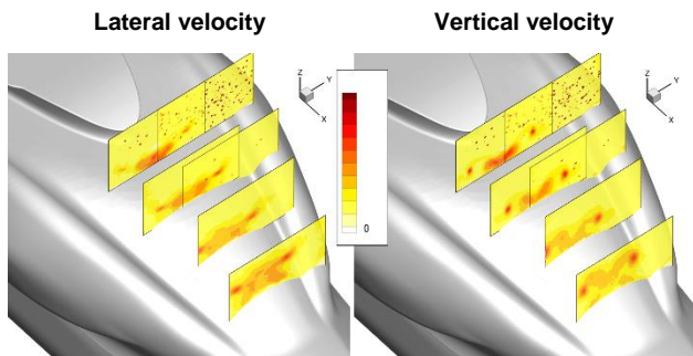
Figure 18 – RMS velocity field in the PIV planes; Configuration AI_NONE, AoA = 0°, AoY = 0°, U = 40 m/s
