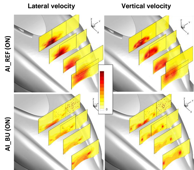
Figure 27 – RMS velocity field in the PIV planes; Operating air intakes ; AoA = 0^\circ , AoY = 0^\circ , U = 40 m/s
