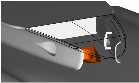
Figure 6 – Air intake #1 (AI_REF) located at the aft portion of the pylon fairing
