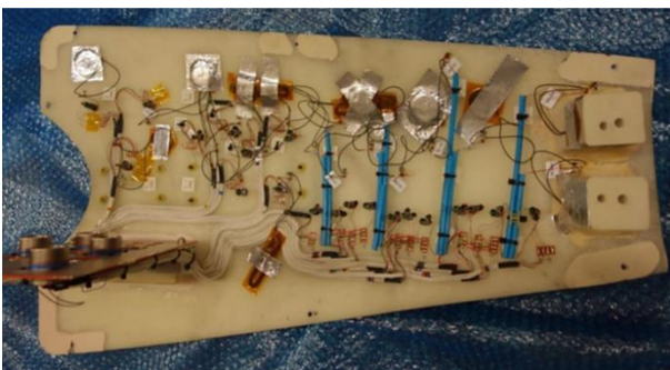
Figure 15 – Internal side of the rear cowling equipped with pressure sensors
