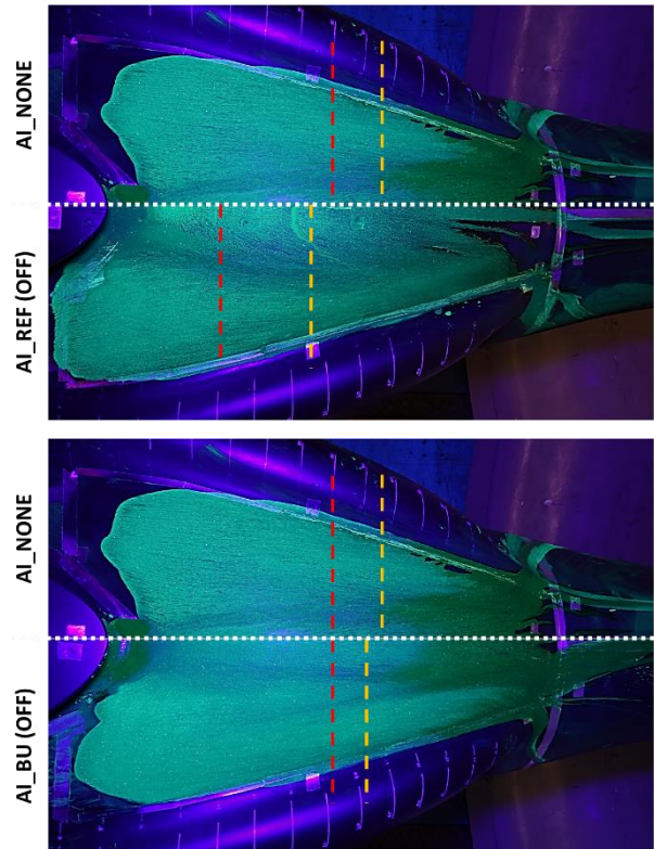
Figure 22 – Locations of the mean flow-separation for AoA = 0°; Rear-central separation in yellow; Lateral separation in red; Top: Configuration AI_REF; Bottom: Configuration AI_BU; AoY = 0°, U = 40 m/s
