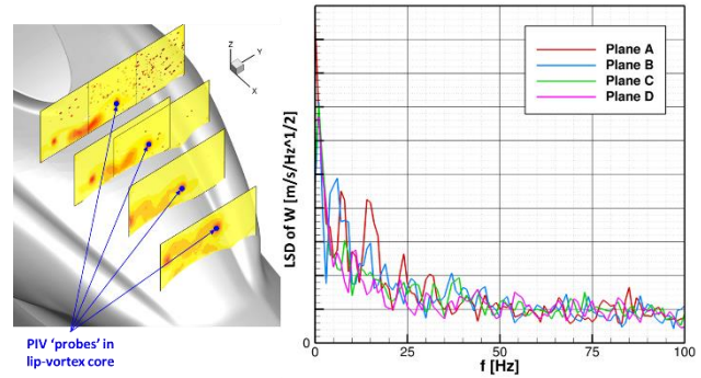
Figure 19 – Left: RMS vertical velocity field in the PIV planes with probes located in the lip-vortex core; Right: Linear spectral density (LSD) of the vertical velocity component in the lip-vortex core in all PIV planes; Configuration AI_NONE, AoA = 0°, AoY = 0°, U = 40 m/s
