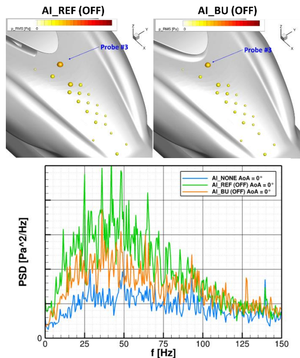
Figure 23 – Top: RMS pressure at the skin pressure sensors; Bottom: PSD of static pressure at probe #3; AoY = 0°, U = 40 m/s
