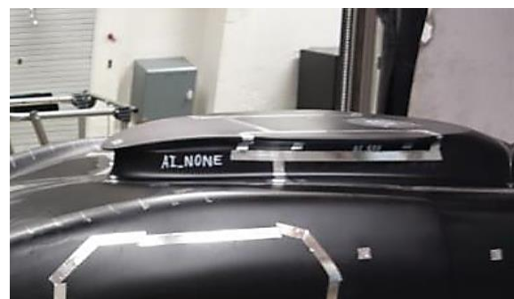
Figure 5 – Baseline pylon-fairing shape with no APU air intake (AI_NONE)
