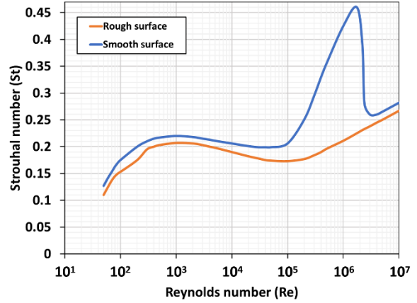
Figure 10 – Strouhal number as a function of the Reynolds number for circular cylinders, from [10] and [1]
