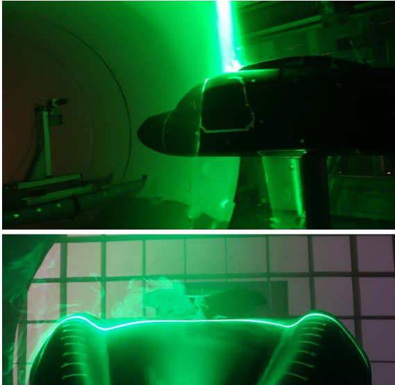
Figure 13 – General view of the PIV system during acquisition
