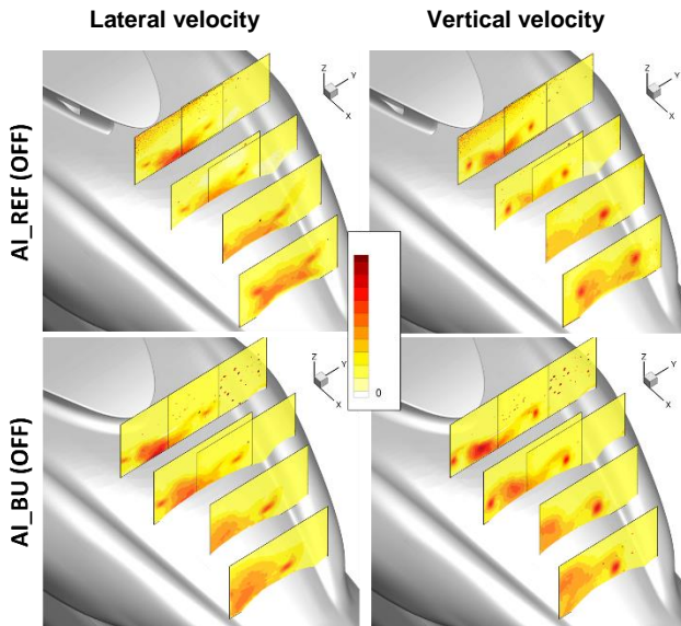
Figure 24 – RMS velocity field in the PIV planes; Non-operating air intakes, AoA = 0^\circ , AoY = 0^\circ , U = 40 m/s
