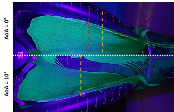
Figure 20 – Locations of the mean flow-separation for AoA = 0° and 10°; Rear-central separation in yellow; Lateral separation in red; Configuration AI_NONE, AoY = 0°, U = 40 m/s
