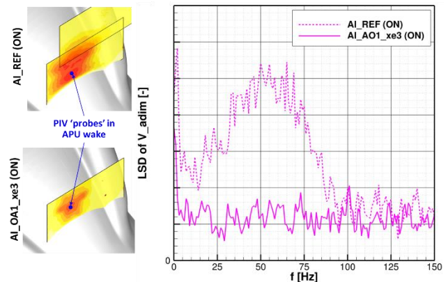
Figure 32 – Left: RMS lateral velocity field in the PIV plane D with probes located at the maximum RMS level; Right: Linear spectral density (LSD) of the lateral velocity component in APU wake; Configuration AI_REF and AI_OA1_xe3, operating APU, AoA = 0°, AoY = 0°, U = 40 m/s
