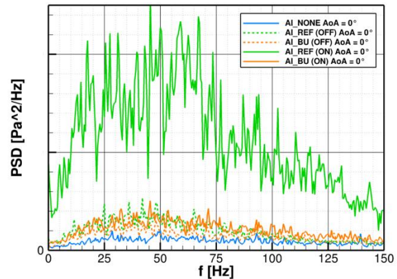
Figure 25 – Top: RMS pressure at the skin pressure sensors; the sensor sphere radii are sized and colored by RMS pressure; Bottom: PSD of static pressure at probe #3; PSD in off mode are also reported in dotted lines; AoY = 0^\circ , U = 40 m/s
