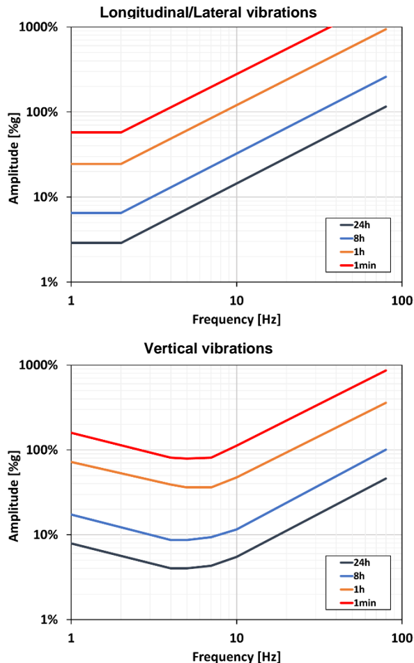
Figure 2 – ISO 2631 daily exposure limits for human response to whole-body vibrations; Amplitudes in % of the Earth's surface standard gravitational acceleration g ; top: longitudinal/lateral vibrations; bottom: vertical vibrations, from [6]
