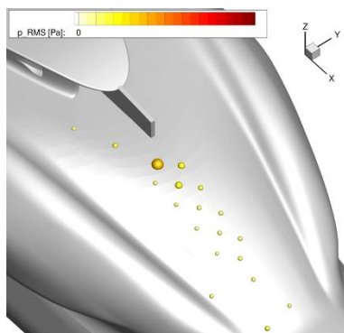
Figure 30 – RMS pressure at the skin pressure sensors for AI_OA1_xe3 configuration at AoA = 0°; the sensor sphere radii are sized and colored by RMS pressure; AoY = 0°, U = 40 m/s
