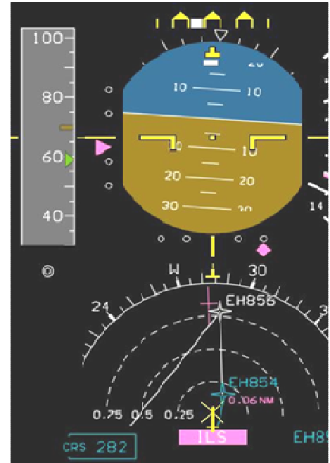
Figure 2 RNAV-ILS and ILS-one guidance display
