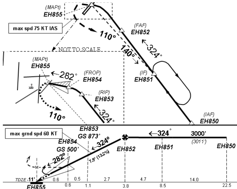
Figure 1 Steep curved final approach procedure
