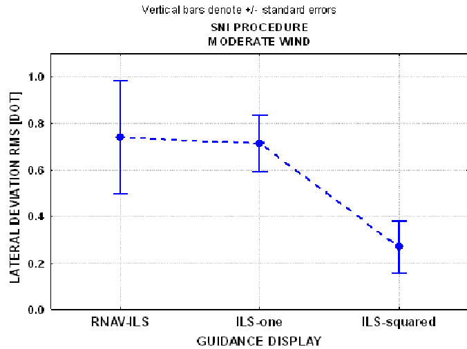
Figure 19 Effect of guidance display on lateral deviation RMS. SNI procedure; moderate wind
