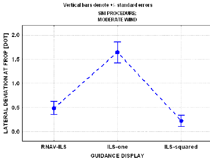
Figure 20 Guidance display main effect on lateral deviation at the FROP. SNI procedure; moderate wind
