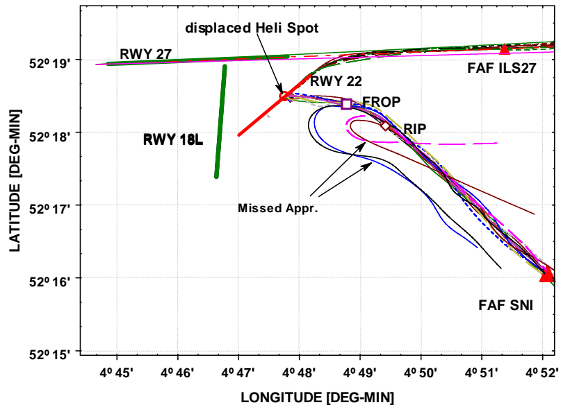
Figure 13 Flight tracks for the baseline and SNI procedures
